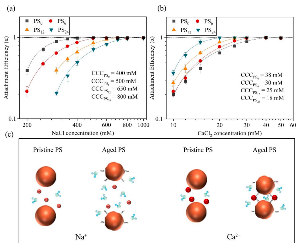
Fig. 1. The aggregation kinetics of pristine and aged PS NPs in NaCl (a) and \text{CaCl}_2 (b) solutions; Schematic diagram of the effect of photoaging on the stability of PS NPs (c). Subscripts 0, 6, 12 and 24 mean aging times of 0, 6, 12 and 24 h.
