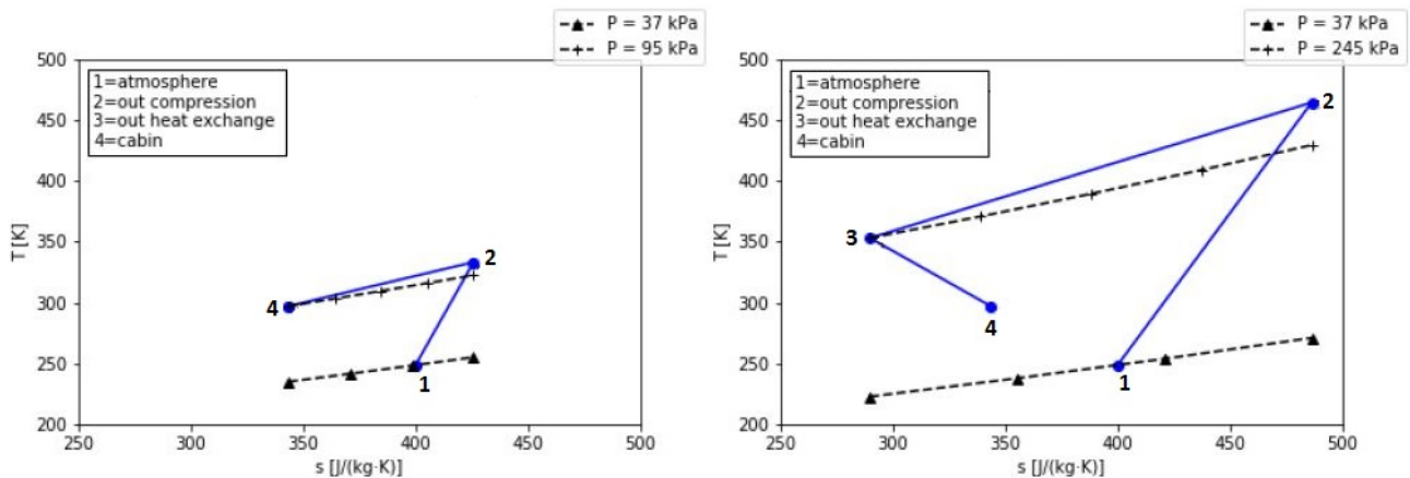
Figure 6 – Two optimised scenarios for the primitive cycle: left - cycle optimised for minimum exergy destruction; right - cycle optimised for best coefficient of performance; standard-day cruise altitude.
