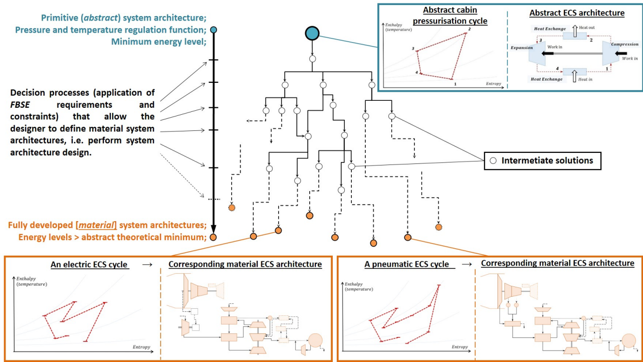
Figure 9 – Schematic overview of the proposed architecture design process spanning the fundamental abstract description on the one end and a variety of possible material architectures on the other.
