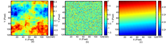
Fig. 5. Simulated residual atmospheric phases after corrections and the orbit phases (one realization). (a) Residual ionospheric phase. (b) Residual tropospheric phase. (c) Orbit error phase.
