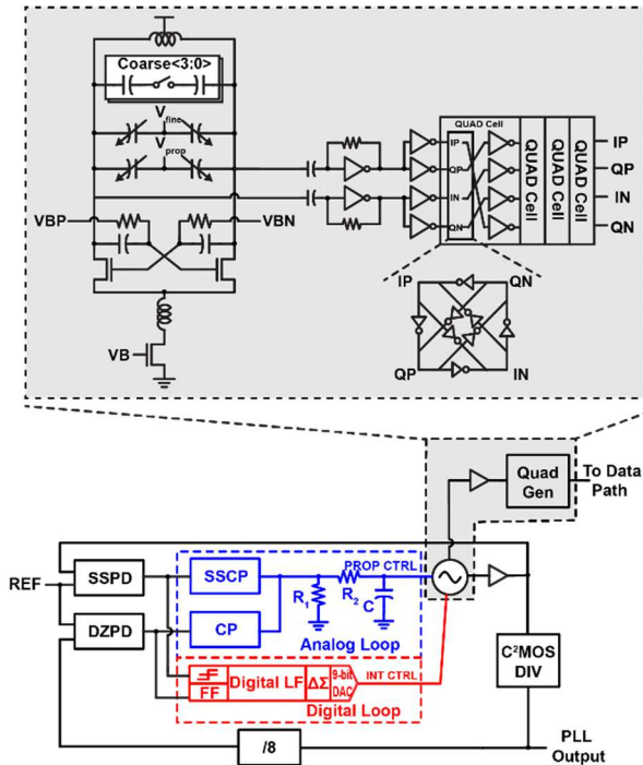
Fig. 2 Structure of hybrid SSPLL and quadrature clock generation.
