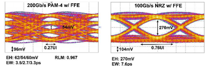
Fig. 7 Eye-diagram of NRZ pattern and PAM-4 pattern
