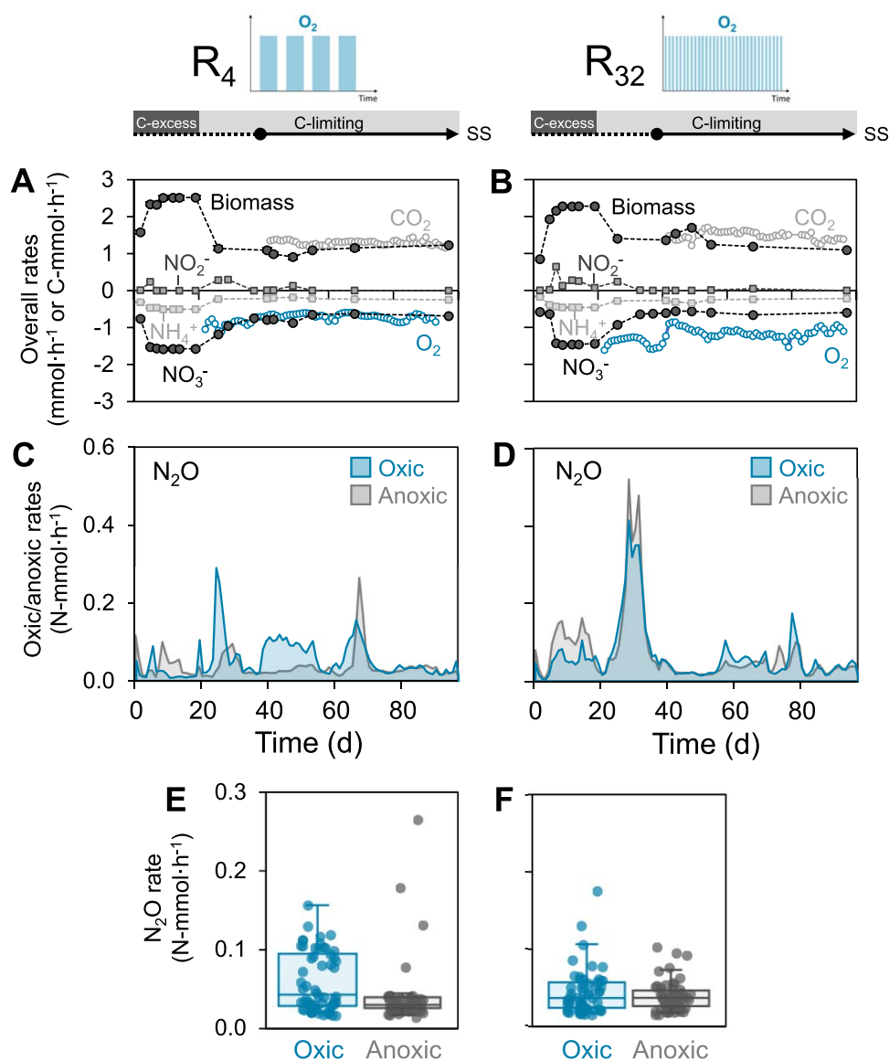
Figure 1. Conversion rates (mmol·h -1 ) in the low- (R 4 ) and high-frequency (R 32 ) oxic/anoxic cycling reactors over the entire operational period. Prior to the target carbon limiting conditions, the reactors were started up for 20 days under carbon excess. The steady state (SS) was reached on day 37 and maintained for over 2 months (equivalent to 30 generation times). Negative rates represent consumption whereas positive rates represent production. (A, B) Overall (i.e. combined aerobic and anaerobic) NO 3 - , NH 4 + , and O 2 consumption, and NO 2 - , CO 2 , and biomass production rates (in mmol·h -1 or C·mmol·h -1 for the carbon compounds). The latter was calculated from the NH 4 + consumption rate. For consistency, an ‘overall’ O 2 consumption rate was calculated by averaging its aerobic consumption over the entire cycle duration. Error bars of all rates are smaller than the symbols and represent the standard deviation of triplicate samples (nitrogen substrates) or of daily averages of continuous measurements (CO 2 and O 2 ). (C, D) Daily average N 2 O production rates (N·mmol/h) during the oxic and anoxic phases. (E, F) Boxplots summarising the daily N 2 O emission rates (N·mmol/h) in both phases during the SS period.
