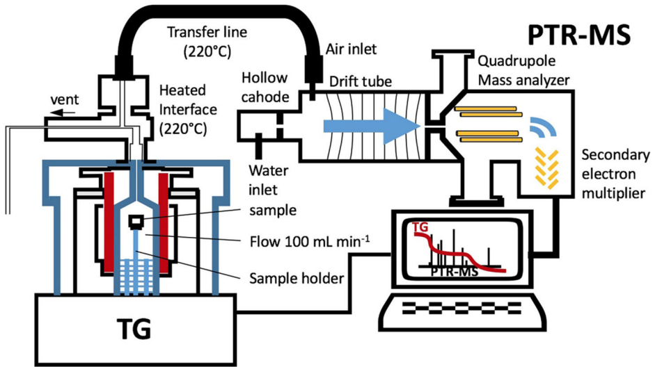
Figure 11. Typical TG-MS analysis system [87].
