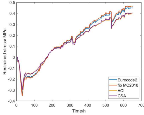
Figure 4-6 Stress results of the mix C3-50 using formulas of elastic modulus of 4 international codes
