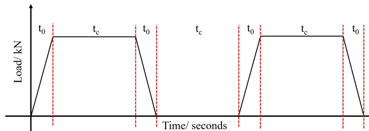
Figure 5-4 Hourly repeated load for elastic modulus/ aging creep test ( t_0 : 30 seconds loading time for testing elastic modulus; t_c : 3600 seconds sustaining at a constant load for testing creep)
