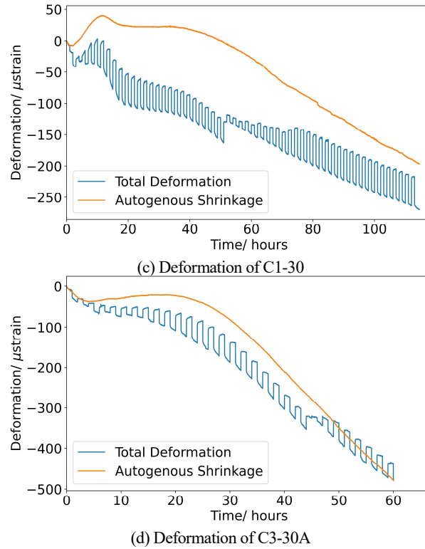
Figure 5-10 Testing results for elastic modulus and creep of CEM I w/b = 0.30: (a-b) Hourly-repeated loading scheme for C1-30 and C3-30A, respectively; (c-d) Deformation results of the test for C1-30 and C3-30A, respectively.
