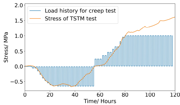
(a) Loading scheme of C1-30
