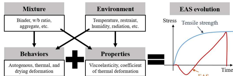
Figure 1-1 Schematic figure for EAS evolution and EAC
