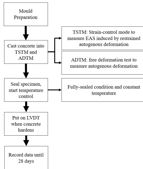
Figure 3-2 ADM and TSM testing procedure
