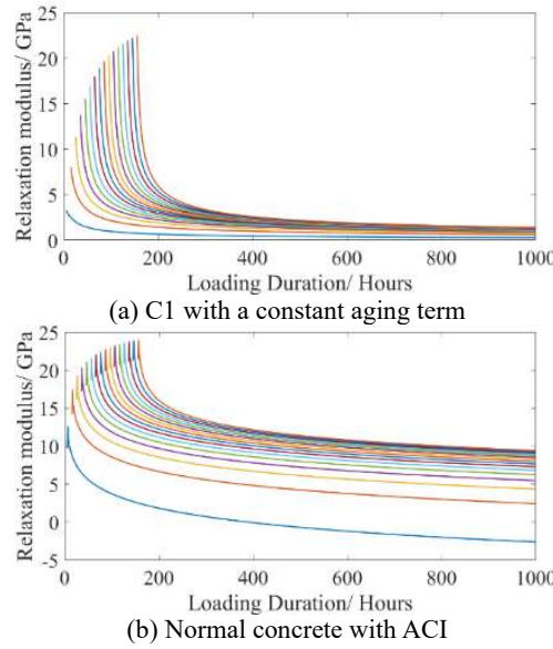
Figure 7-8 Relaxation modulus R(t_0, t) converted from creep compliance function by M1 for: (a) C1 creep compliance function with a constant aging term; (b) ACI-based creep compliance function for normal concrete as used in [212].
