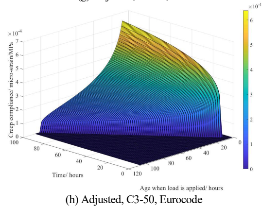
Figure 4-17 Original and adjusted creep compliance function: (a-b) original creep compliance function of C3-35 of ACI and Eurocode; (c-d) original creep compliance function of C3-50 of ACI and Eurocode; (e-f) adjusted creep compliance function of C3-35 of ACI and Eurocode; (g-h) adjusted creep compliance function of C3-50 of ACI and Eurocode;
