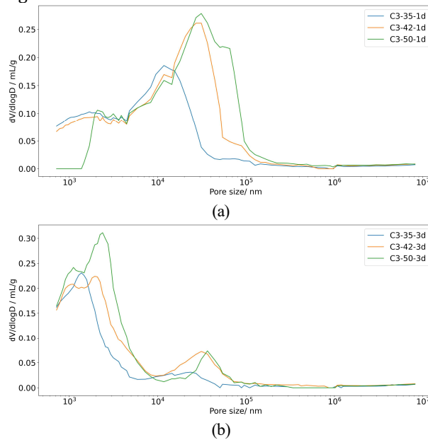
Figure 3-14 Pore size distribution at ages of: (a) 1 day; (b) 3day
