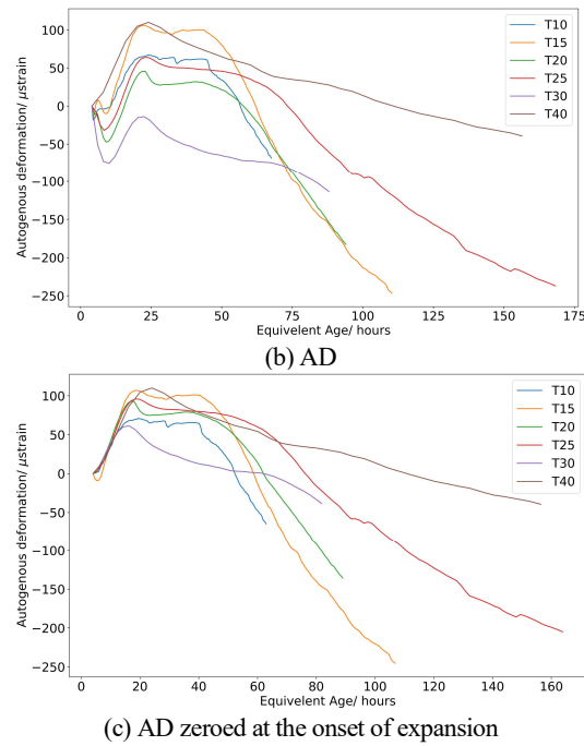
Figure 6-2 The AD and EAS of cement paste with respect to the equivalent age calculated by the MC: (a) EAS; (b) AD ; (c) AD with the time-zero being the onset of autogenous expansion
