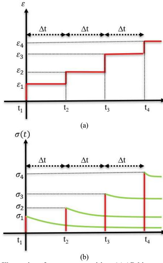
Figure 4-1 Illustration of stress superposition: (a) AD history; (b) Stress of each time interval
