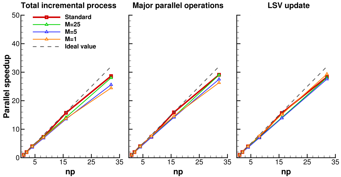
Fig. 7. The speedup of standard and enhanced parallel incremental SVDs for the total incremental time, major parallel operations and LSV update for a 320000 \times 50 synthetic matrix. np denotes the number of processors.
