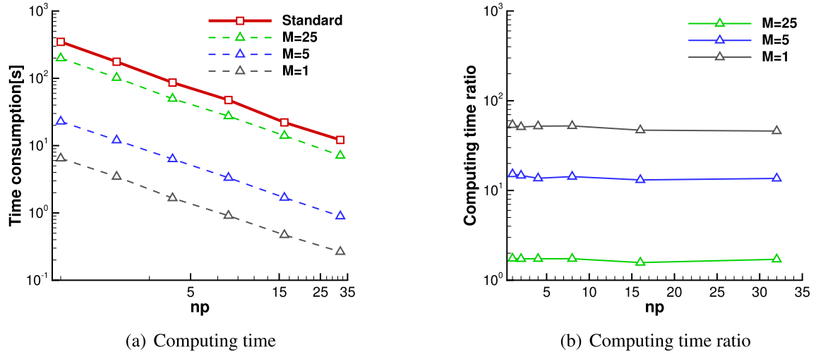
Fig. 6. Time consumption of standard and enhanced incremental SVDs in parallel for a 320000 \times 50 synthetic matrix, and the computing time ratio for these enhanced iSVDs. np denotes the number of processors.
