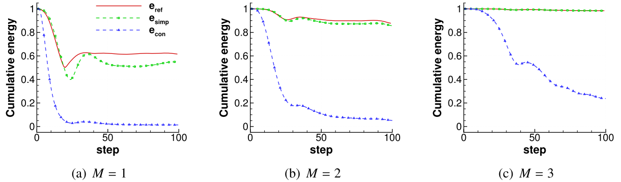
Fig. 4. Cumulative energy computed by estimators, e_{con} and e_{simp} , and reference value from the standard incremental SVD during incremental process for first three truncation numbers ( M ) of the enhanced process.
