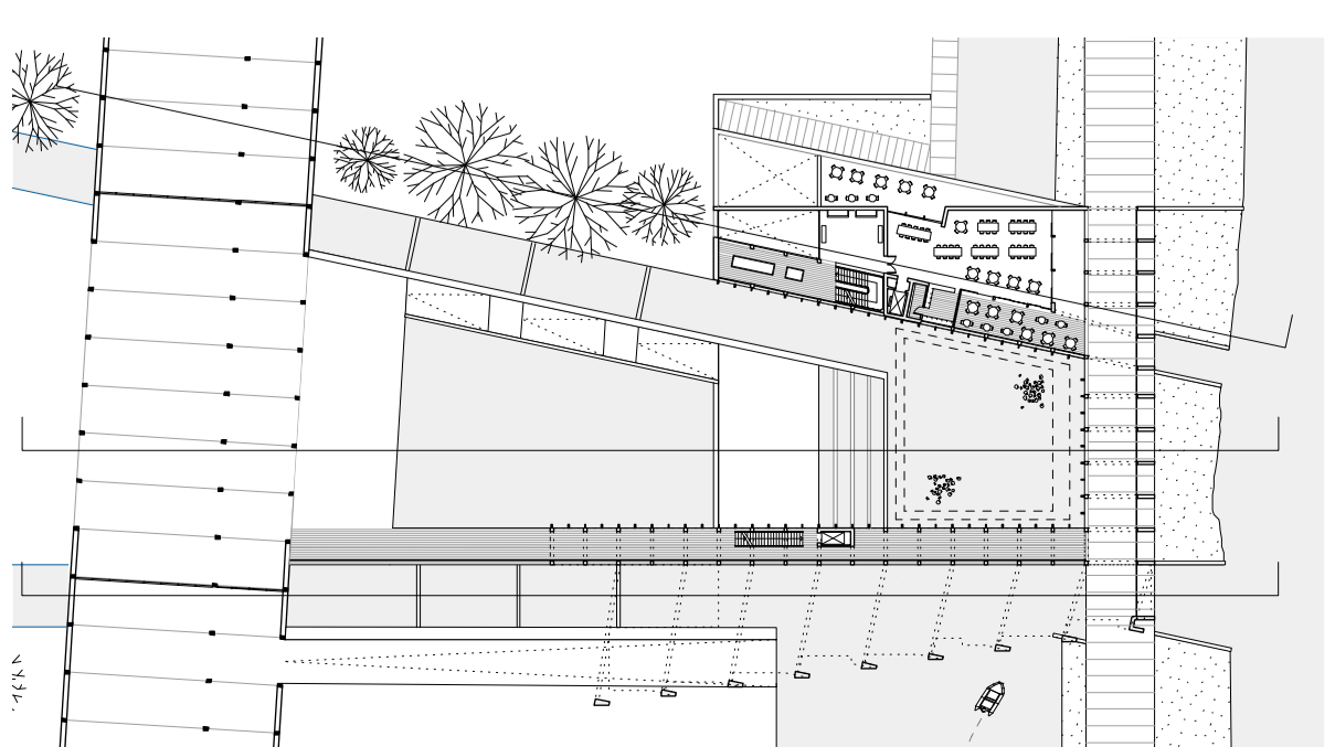
Long section: outdoor courtyard and leisure pool
