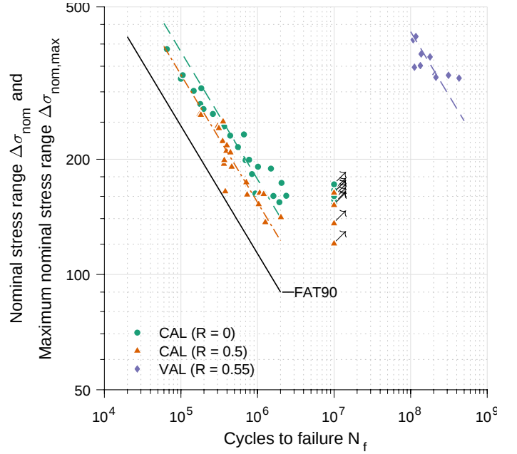
FIGURE 5: FATIGUE TEST RESULTS OF AN EXEMPLARY SCALED BUTT JOINT IN THE OWT SUPPORT STRUCTURE OF THE CASE STUDY UNDER CAL AND VAL AT ROOM TEMPERATURE; CAL RESULTS FROM [29, 30]
