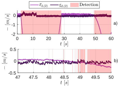
Figure 2.5: Detection of the attack by the observer error based detector. Second element of the observer error bounds. a) whole time range. b) around time of first detection of slope attack.
