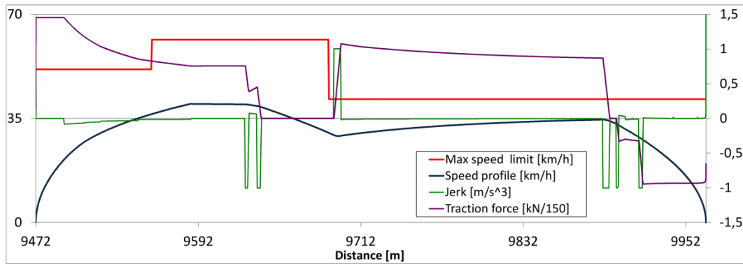
Figure 2-6. Jerk limitation
