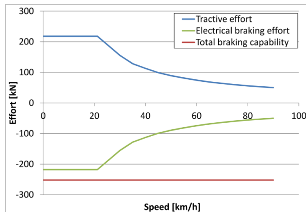
Figure 2-5. Traction/Braking curves
