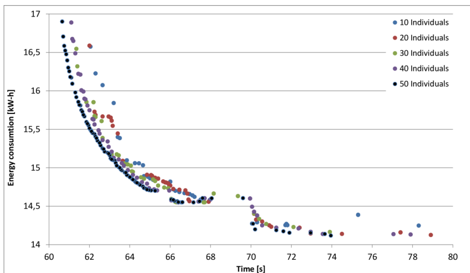
Figure 3-21. Convergence for different population size
