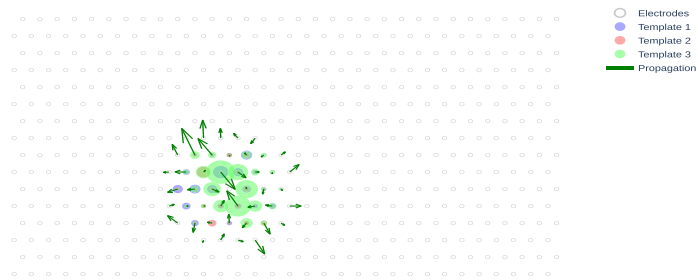
Figure B6. Dynamics of the artifact on MEAs. The arrows show the direction in which each electrode's measured activity is propagated according to A_a x . The shaded colors on the electrodes show the absolute values of B_a , which determines how three input templates of the EI model change the activity of the electrodes.
