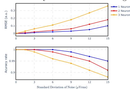
(b) Root mean square error (RMSE) between the estimated inputs and their input templates (top) and spike sorting accuracy (bottom) using synthetic data for multiple neurons firing at different levels of noise measurement.
