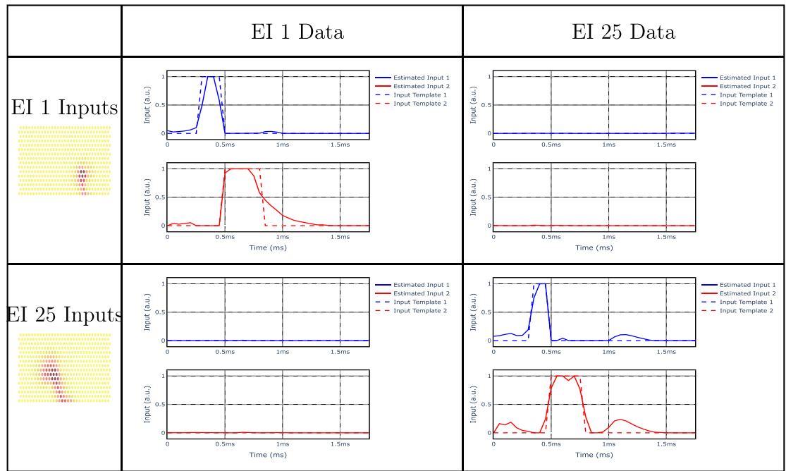
Figure 13. Comparison between retrieved inputs and input templates when ex vivo recordings from EI 1 and EI 25 are fed to the input estimator.
