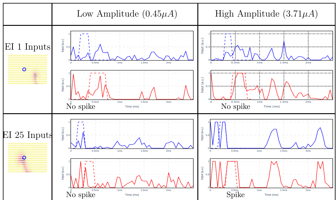
Figure 14. Retrieved inputs of neuron 25 and neuron 1 when ex vivo stimulation data is fed to the input estimator at low amplitude ( 0.45\mu A ) and high amplitude ( 3.71\mu A ). Input templates for each neuron are shown in dashed lines. Neuron 25 is located behind the stimulating electrode (indicated by a circle), and neuron 1 is further away. Using a similarity function, a spike is detected only for neuron 25 at high stimulation amplitude (bottom-right panel).
