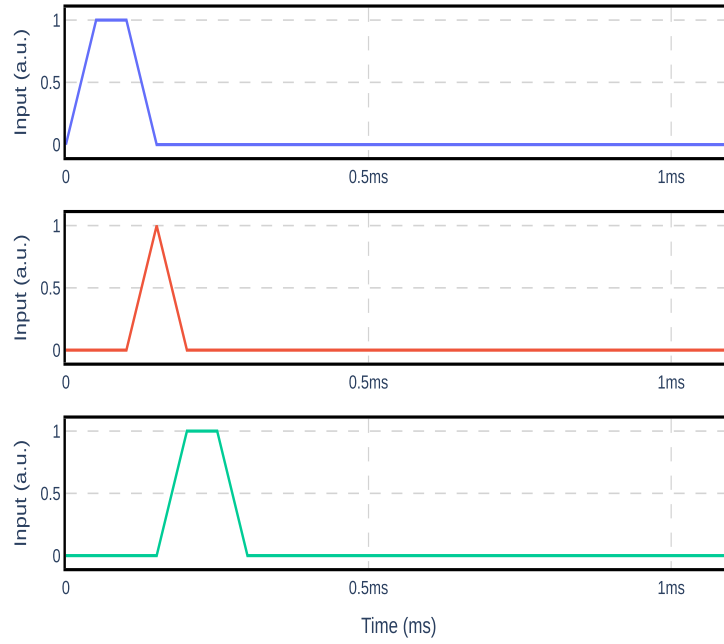
Figure B5. Input templates r'_a of artifact. The blue, red, and green graphs are the first, second, and third entries of the vector r'_a , respectively.
