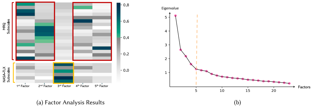
Fig. 5. (a) Factor Analysis Results (b) Scree Plot.
