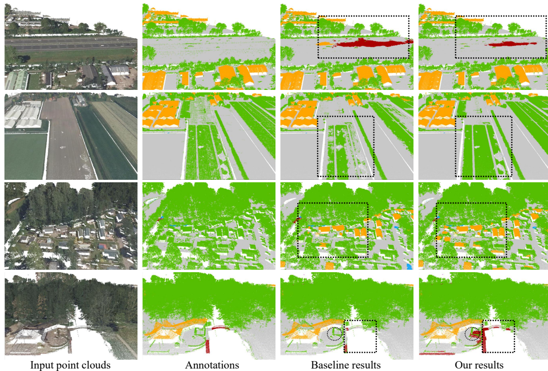
Figure 2. Qualitative results achieved on the AHN dataset, using height and intensity as input features. We use the following color schemes to render the scenes: ■ for building , ■ for ground , ■ for high-tension , ■ for water , ■ for civil structure , and ■ for other . Since AHN is a real-world dataset, its annotations may contain noise and errors. Our improvements are highlighted with black-dotted boxes. Minor segmentation noise in some local regions is marked by black-dotted circles.
