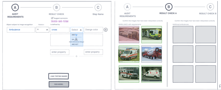
Figure 8: Low-fidelity mock-up used in the co-creation sessions: query functionality and the result interface after a query.
