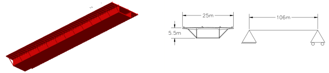
Figure 19 One bridge span subsystem
