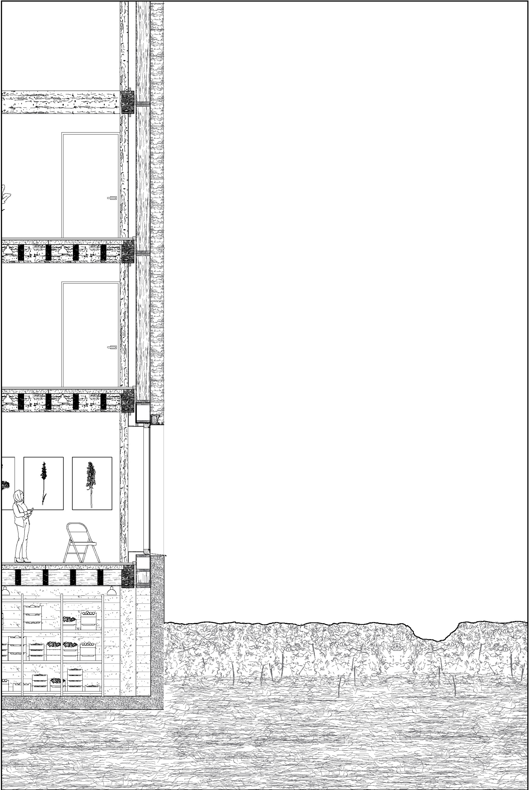
Section, Picture Window 1:50
