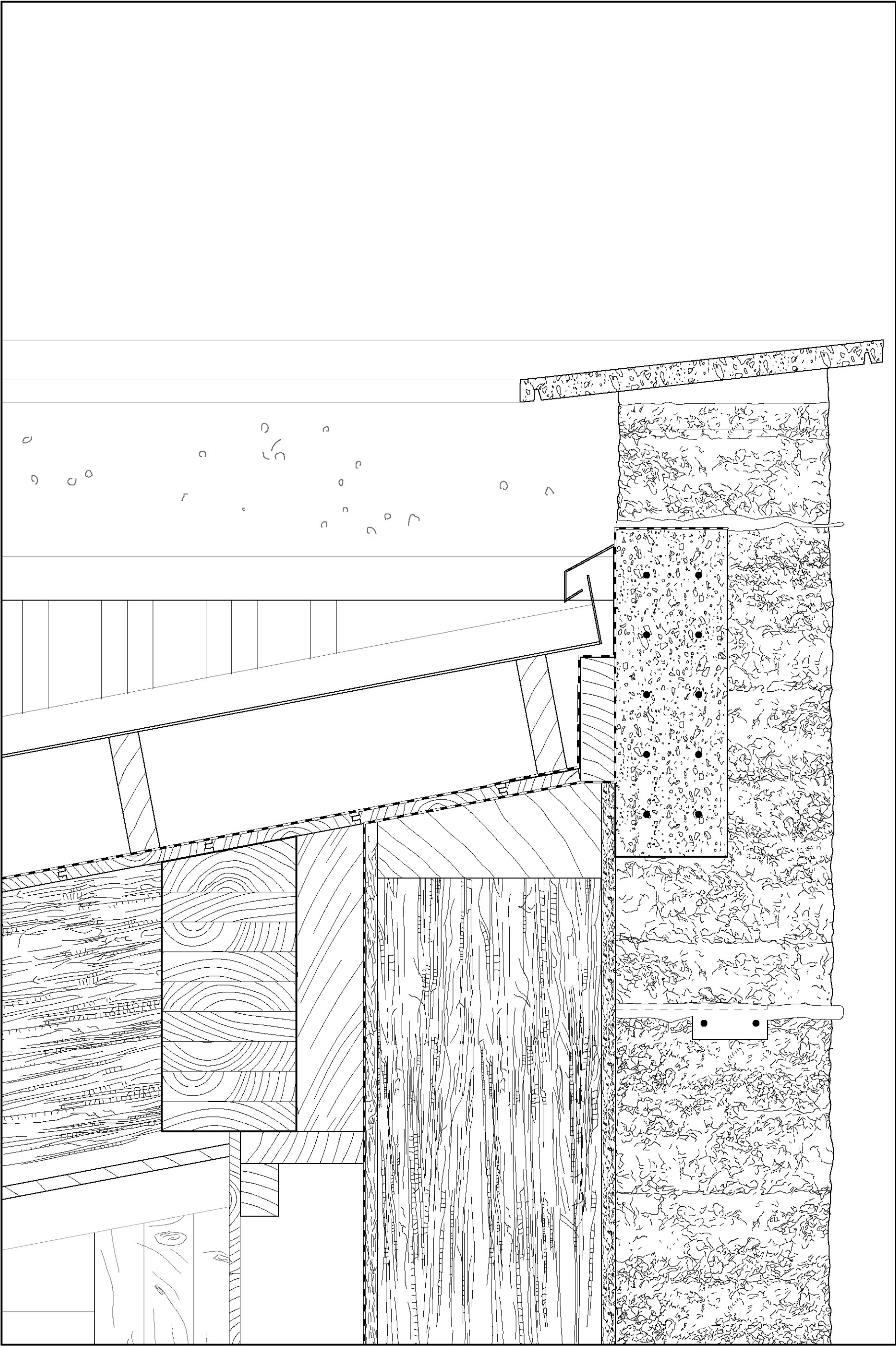
Roof Detail 1:5
