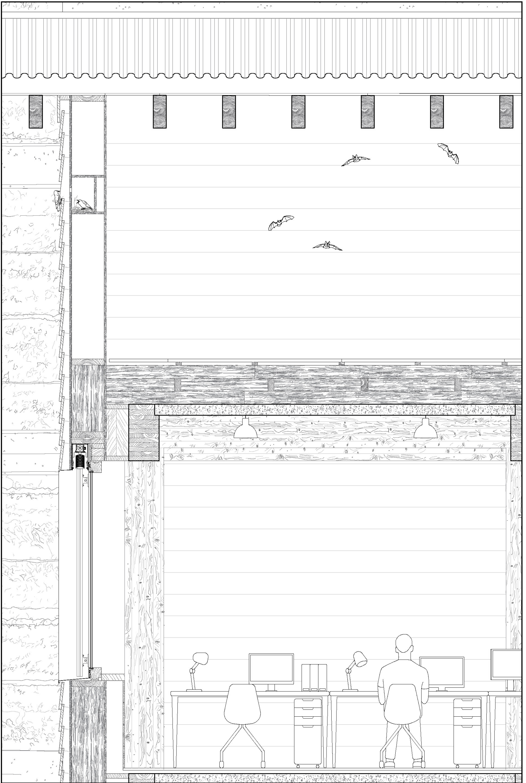
Technical section, cold roof space 1:20
