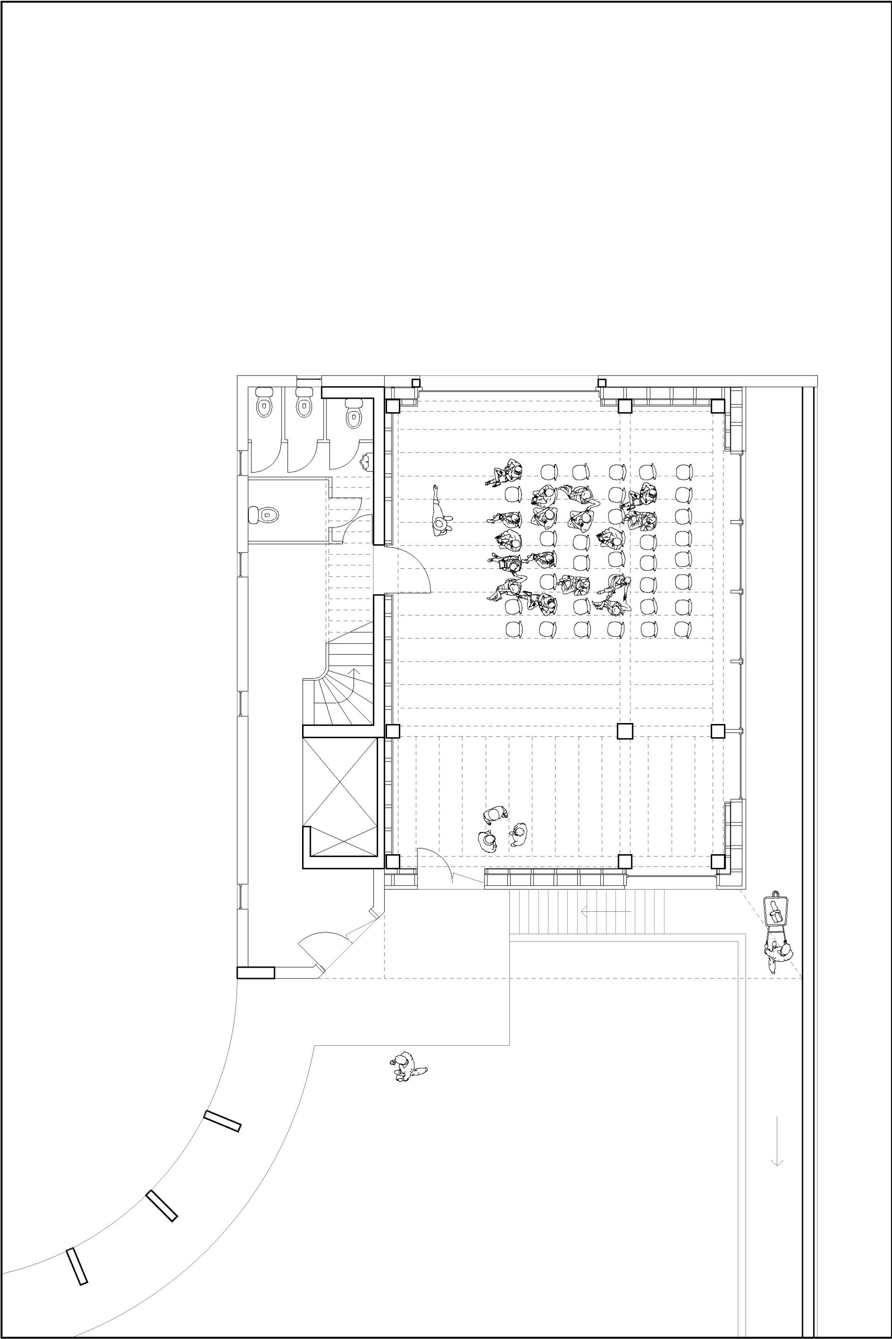
Floorplan ground floor, Public room 1:100
