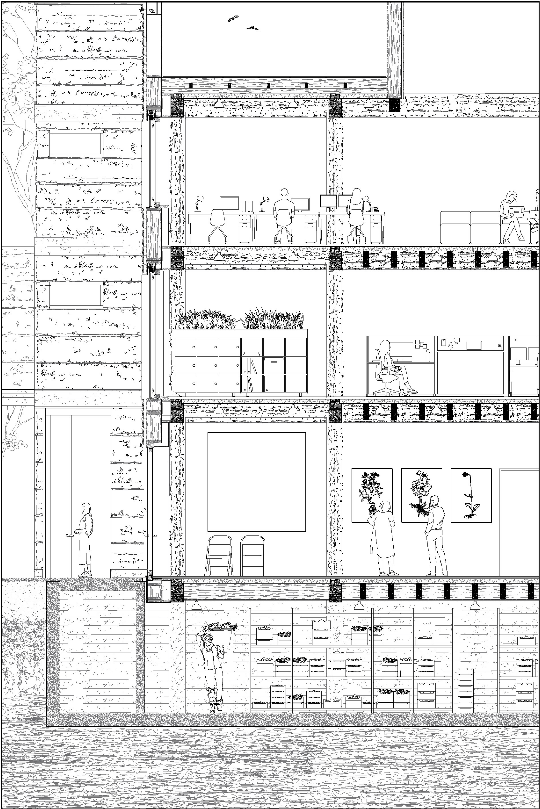
Section, Villa 1:50
