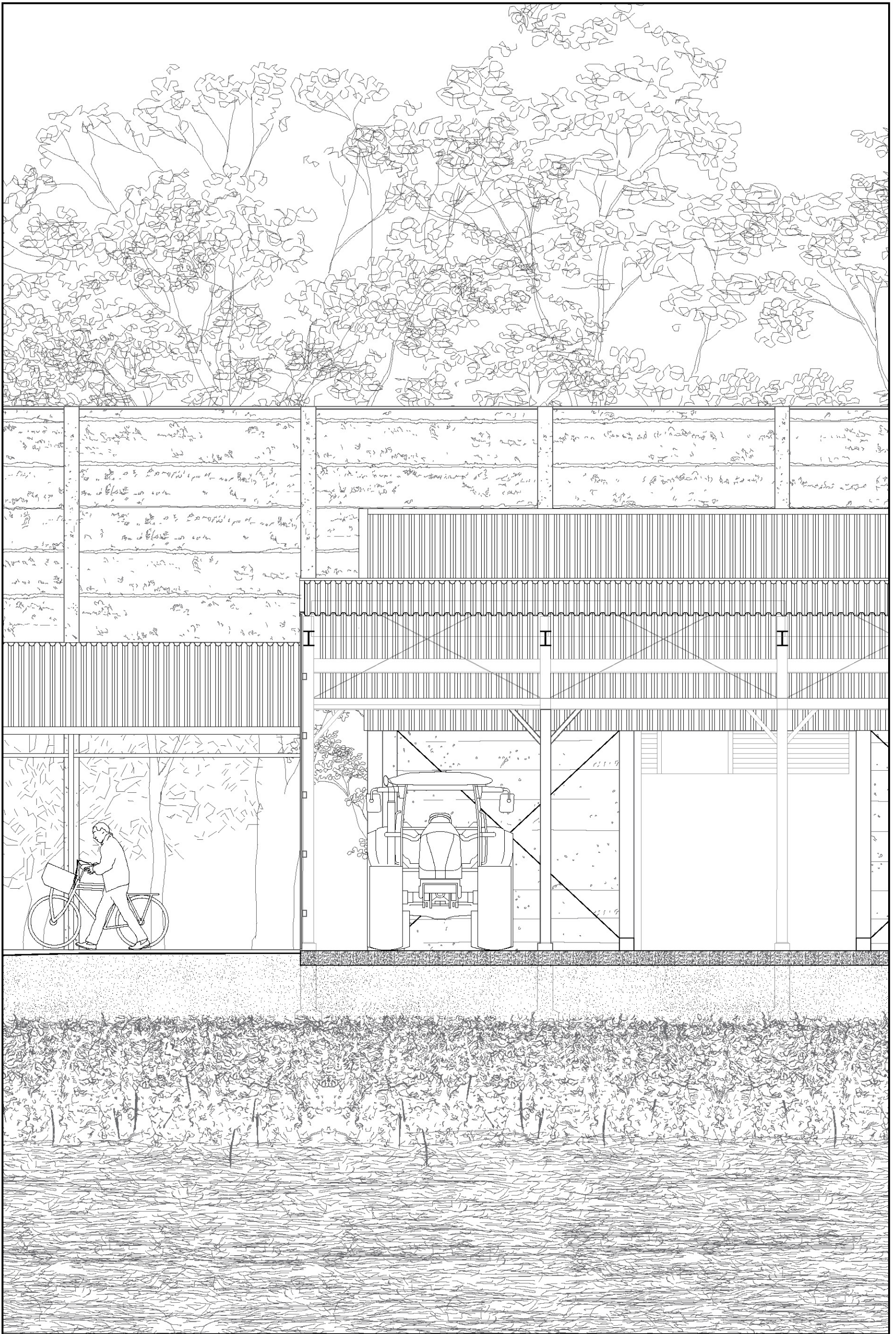
Section, Sheds 1:50
