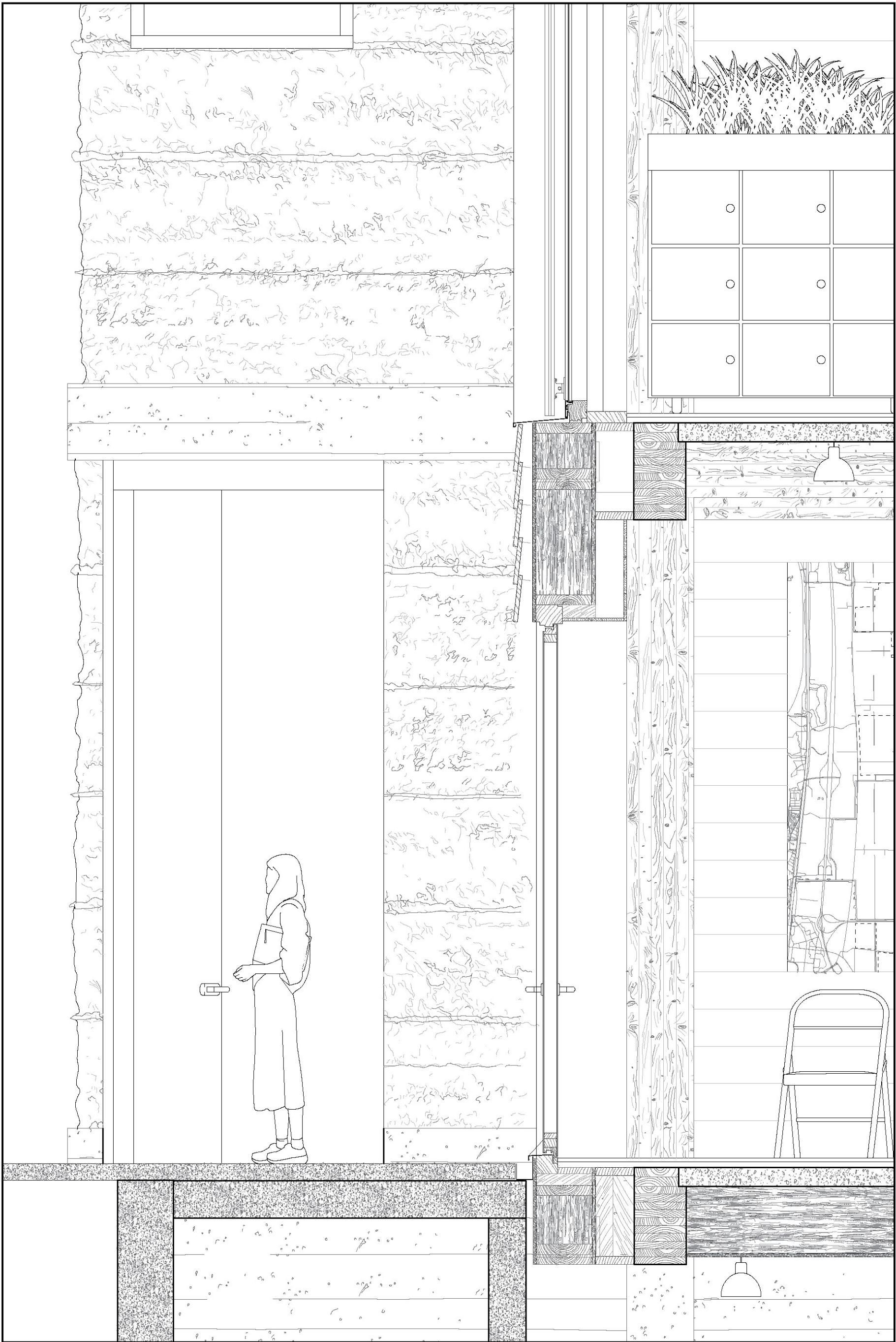
Technical Section, entrance
