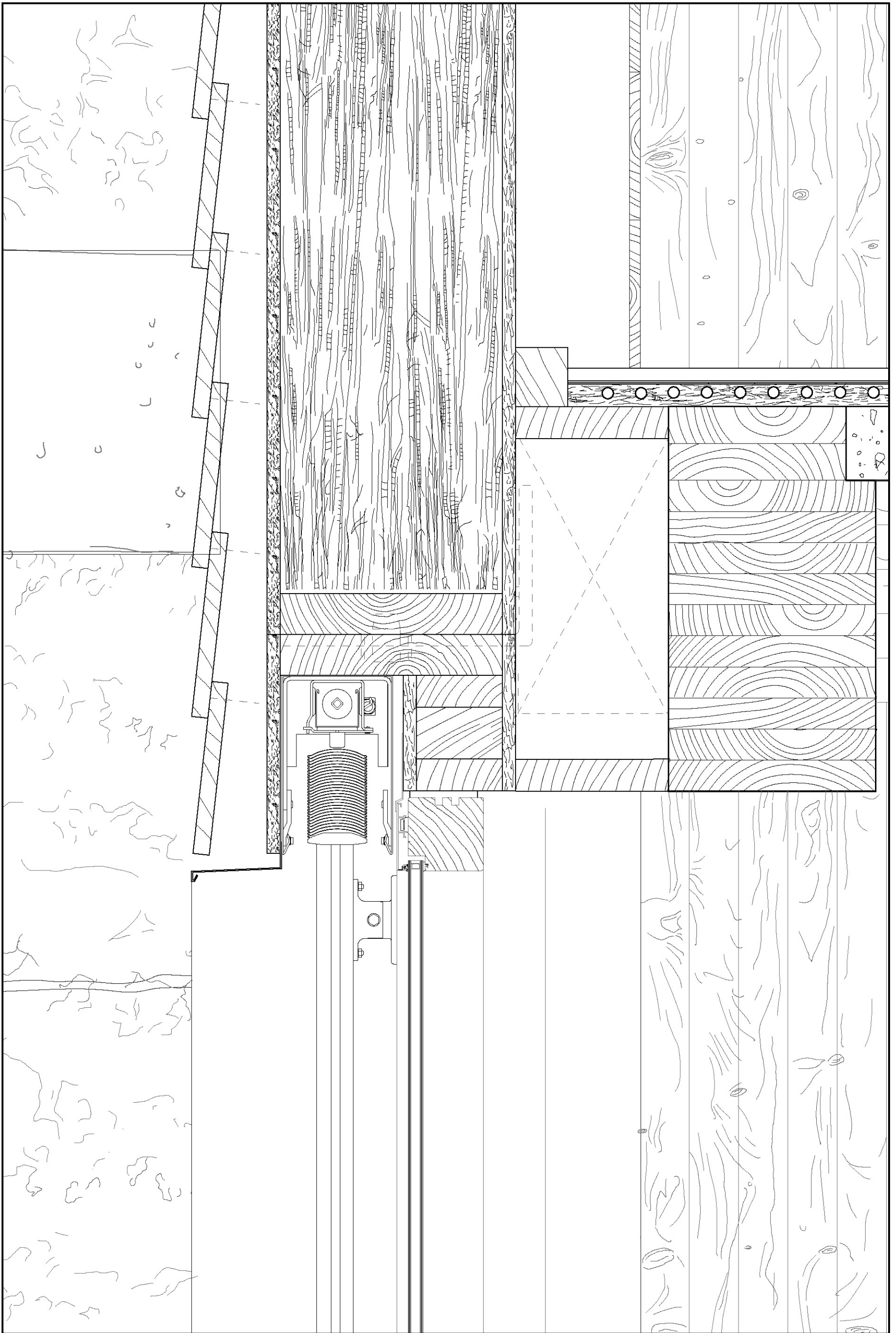
Window Detail 1:5
