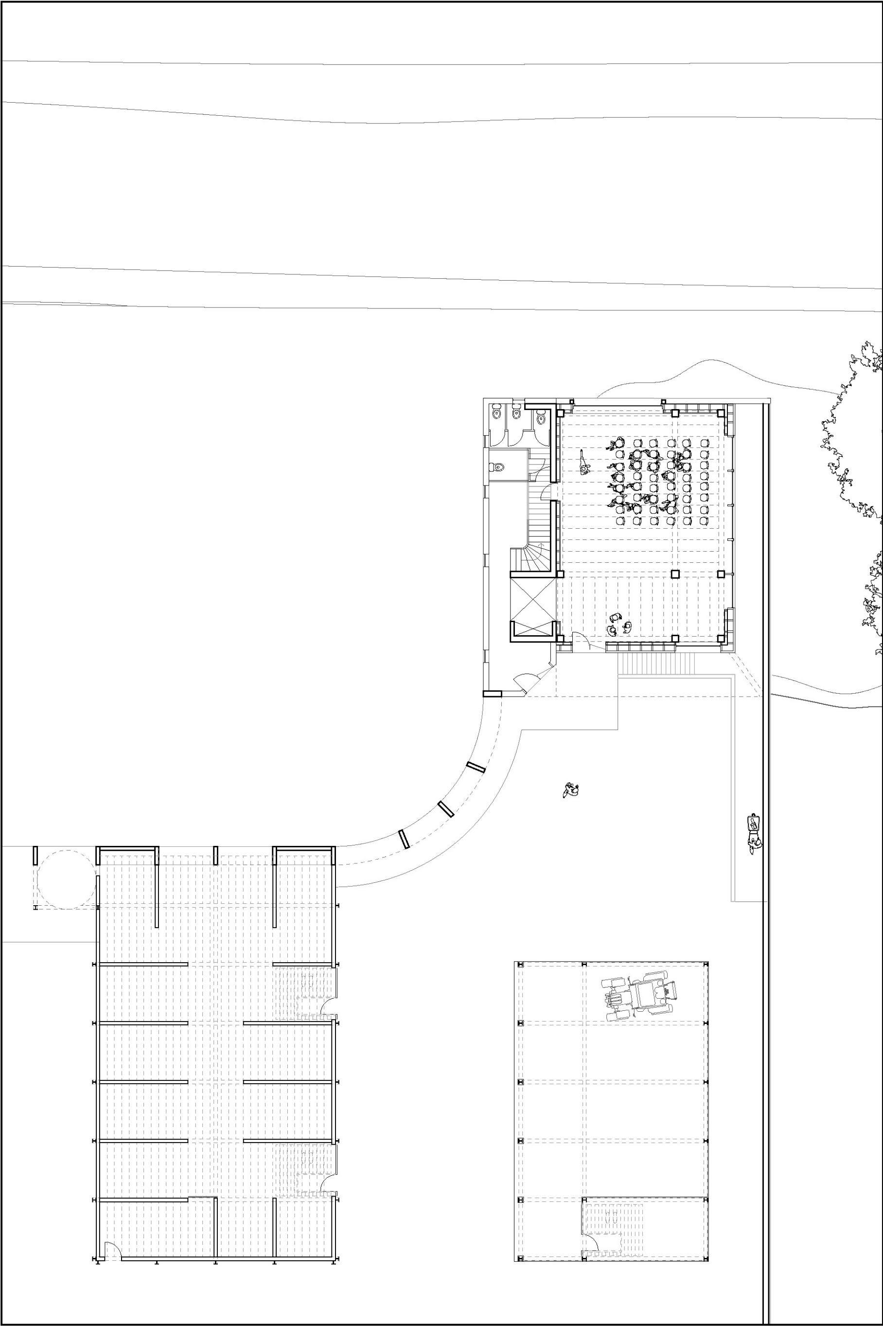
Floorplan Public Room, Sheds 1:200
