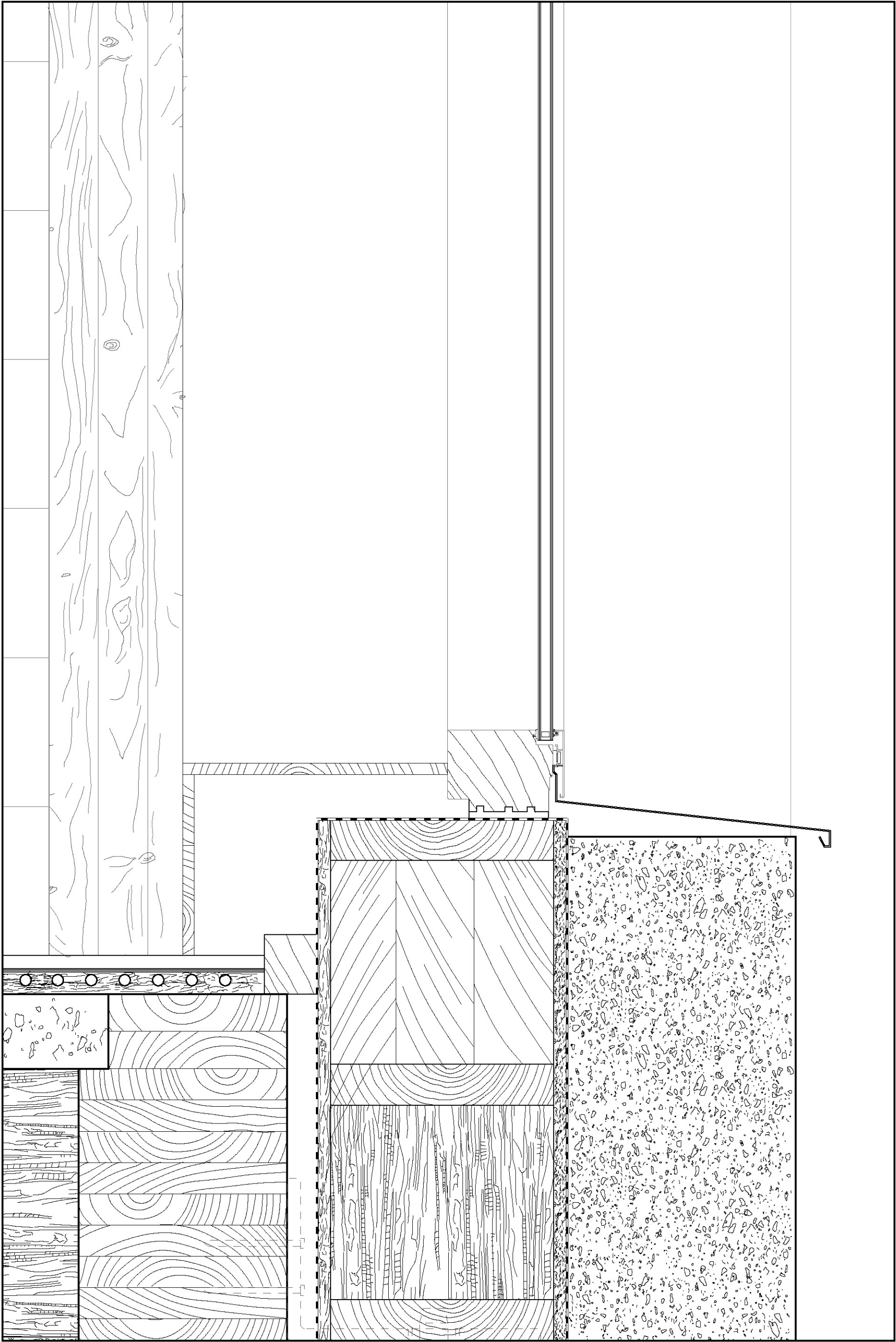
Picture Window Detail
