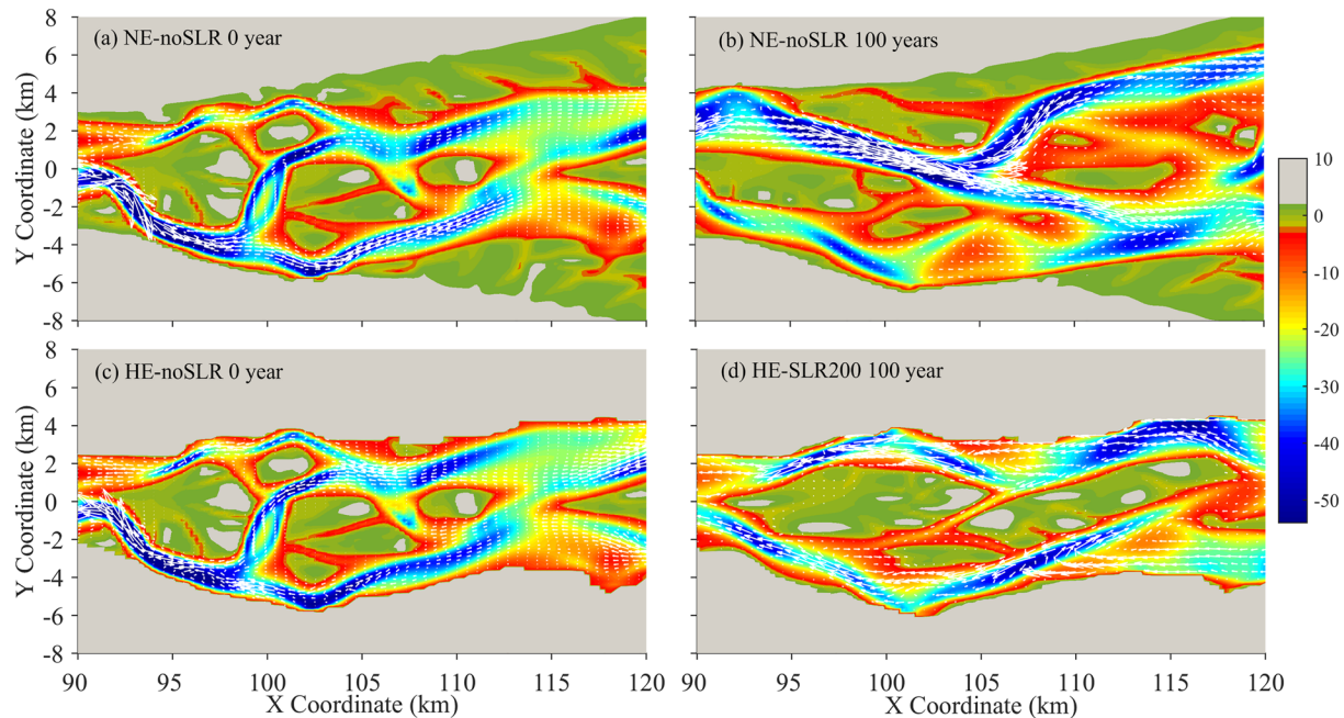
Figure 10. Distribution of the tidally averaged sediment transport vectors in a selected segment of the basin (km-90 to km-120) at the beginning and end of the 100-year simulations, with the bathymetry in the background: (a) NE-noSLR at the beginning, (b) NE-noSLR at the end, (c) HE-noSLR at the beginning, and (d) HE-SLR200 at the end. The length scale of the vectors in panel (c) and (d) is a third of that in panel (a) and (b).
