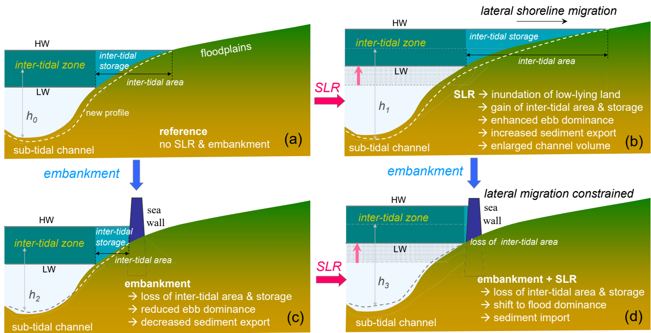
Figure 17. Conceptual sketches showing changes of the half cross-section profile (a) in the reference case, (b) (high) sea-level rise (SLR) scenario, (c) (medium) embankment scenario, and (d) combined embankment and SLR. LW and HW indicate low water and high water, respectively.
