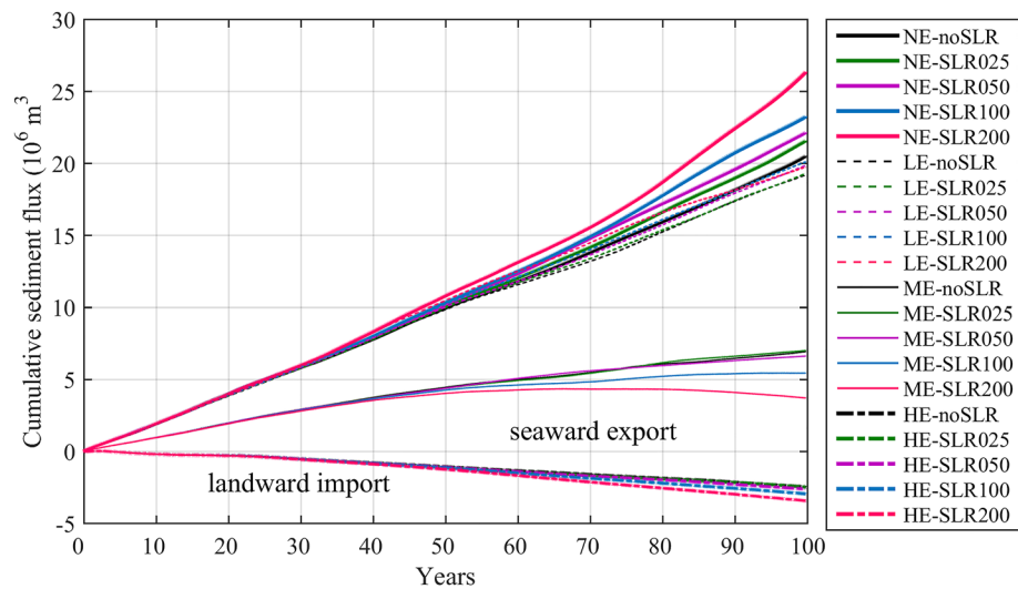
Figure 7. Changes of cumulative sediment flux at the mouth section over 100 years in all sensitivity simulations. Positive values indicate sediment export (seaward flux) and negative values indicate sediment import (landward flux).
