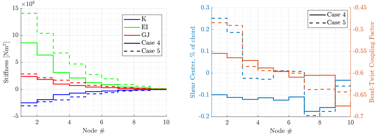
Figure 8: Comparison of stiffness properties of cases 4 and 5.
