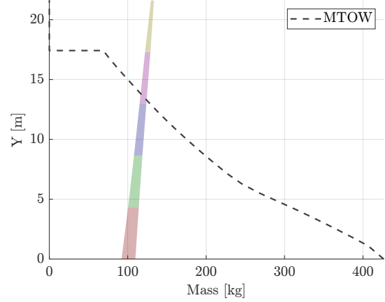
(b) Distribution of fuel mass across the wing in MTOW configuration.
