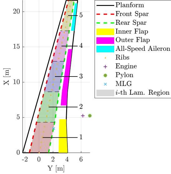
(a) Structural layout, movables layout, non-structural mass distribution, and laminate regions.
