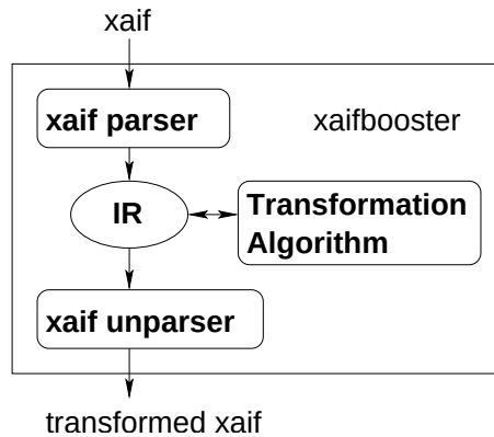
Figure 4: xaifBooster parses xaif code into an internal representation (IR). It provides an API for transformation algorithms to modify the IR. An unparser returns the transformed xaif code.
