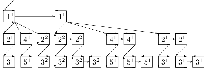
Figure 3: Call tree reversal: code (a), call tree (b), adjoint call tree in split (c) and joint (d) reversal
