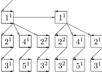
Figure 3: Call tree reversal: code (a), call tree (b), adjoint call tree in split (c) and joint (d) reversal
