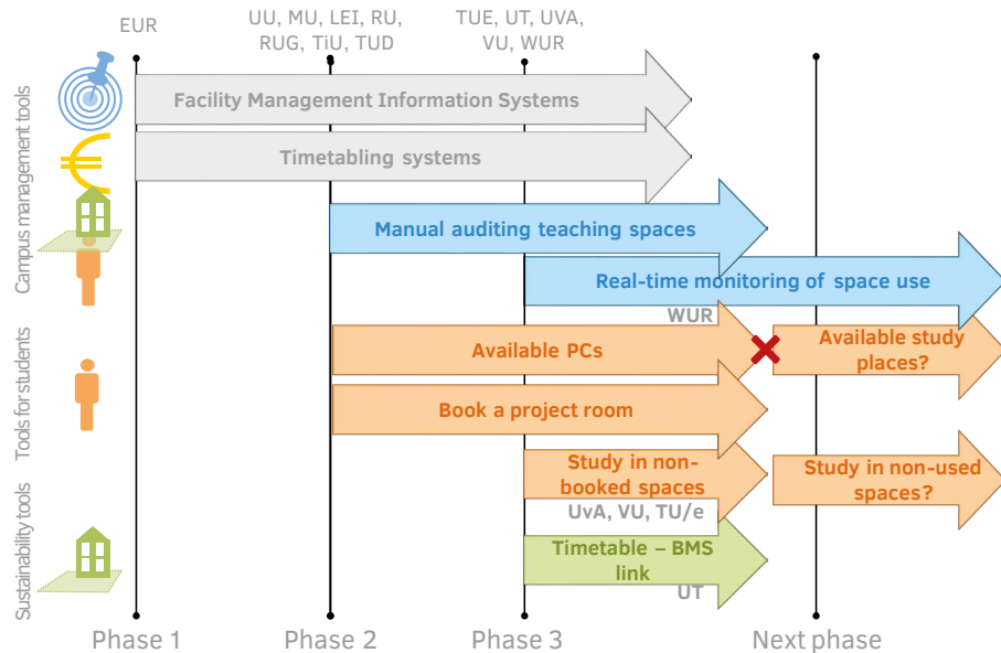
FIG. 6.5 Overview of the available SCTs at Dutch universities in 2016, positioned in time to indicate the development of SCTs.
