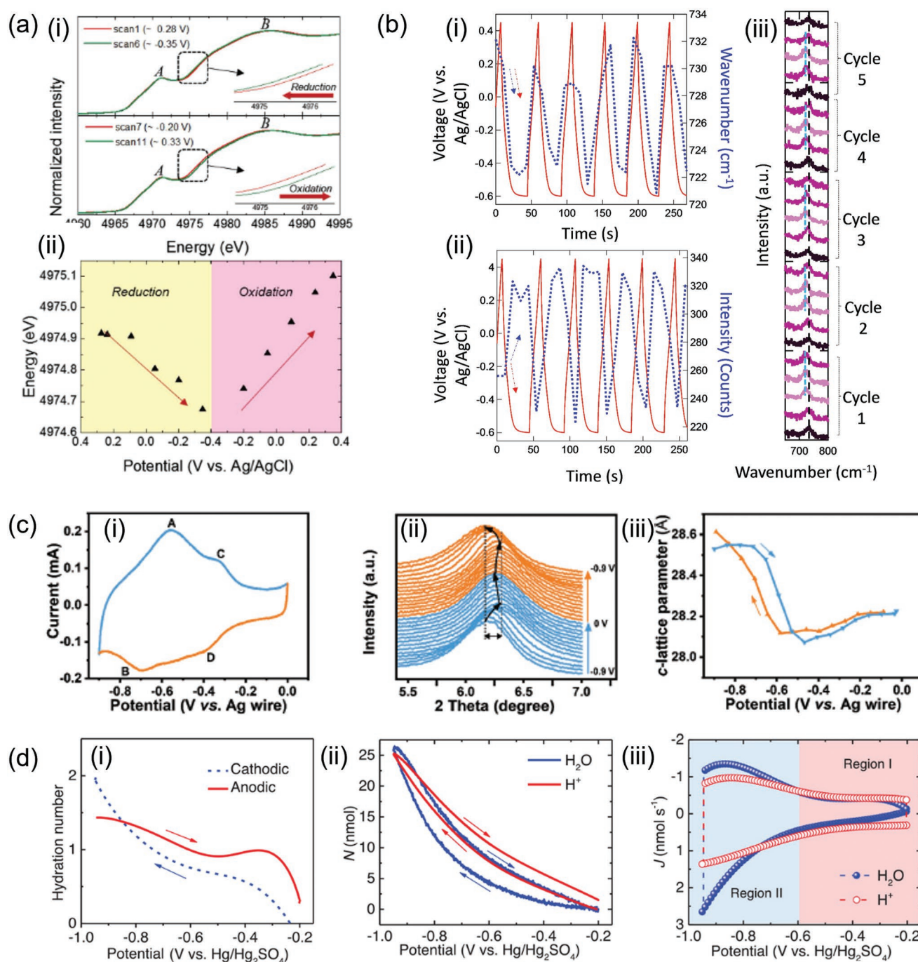
Figure 2. In situ characterization of MXene electrodes in an acidic environment. a) i) Ti K-edge XANES spectra recorded during positive and negative polarization of \text{Ti}_3\text{C}_2\text{T}_x electrode in 1 M \text{H}_2\text{SO}_4 ii), variation of Ti edge energy as a function of the applied potential. Reproduced with permission. [30] Copyright 2015, Wiley b) The changes in the wavenumber i) and the peaks intensity ii) recorded by in situ Raman spectra upon cycling of \text{Ti}_3\text{C}_2\text{T}_x electrodes in 0.1 M HCl, iii) the variation in the recorded spectra during 5 cycles. Reproduced with permission. [32] Copyright 2022, Wiley c) in situ XRD analysis of MXene electrodes in 1 M \text{H}_2\text{SO}_4 : i) CV response, ii) XRD patterns collected during charging/discharging, iii) the corresponding variation in the d spacing with the applied potential. Reproduced with permission. [26] Copyright 2019, Wiley d) in situ EQCM measurements of MXene electrodes in 1 M \text{H}_2\text{SO}_4 solution: i) calculated hydration number of the inserted protons and the total ions population ii) as a function of potential, iii) \text{H}^+ related ionic flux (red) and total ionic flux (blue) versus potential. Reproduced with permission. [35] Copyright 2022, Wiley.
