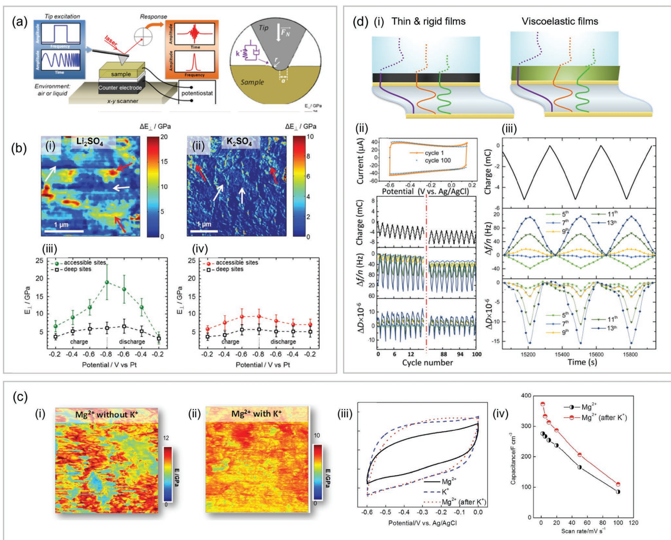
Figure 6. In situ monitoring of mechanical changes in \text{Ti}_3\text{C}_2\text{Tx} electrodes a) Schematic representation of the experimental setup, where the AFM tip vibrates in contact with the sample's surface with a band excitation waveform. b) Elastic modulus mapping of negatively charged ( -0.8\text{ V} ) MXene films immersed in i) \text{Li}_2\text{SO}_4 ii) \text{K}_2\text{SO}_4 electrolytes. Based on the maximal variations in the elastic modulus one can identify the shallow and the deep intercalation sites in the MXene electrodes for both \text{Li}^+ and \text{K}^+ ions insertion (panels (iii) and (iv) respectively). Reproduced with permission. [56] Copyright 2016, Wiley. c) The variations in the elastic modulus of \text{Ti}_3\text{C}_2\text{Tx} after insertion of \text{Mg}^{2+} ions (i) and after pre-cycling in \text{K}_2\text{SO}_4 solutions. (ii). The corresponding changes in the CVs and the rate capability are presented in (iii) and (iv). Reproduced with permission. [43] Copyright 2017, The Royal Society of Chemistry d) i) Schematic descriptions of acoustic wave velocity profiles generated across the quartz crystal, loaded by acoustically thin and thick (viscoelastic) films. ii) CVs, frequency, and dissipation of thick MXene films throughout 100 cycles. iii) An enlarged view of the charge frequency and dissipation changes recorded during 3 cycles. Reproduced with permission. [65] Copyright 2017, American Chemical Society.
