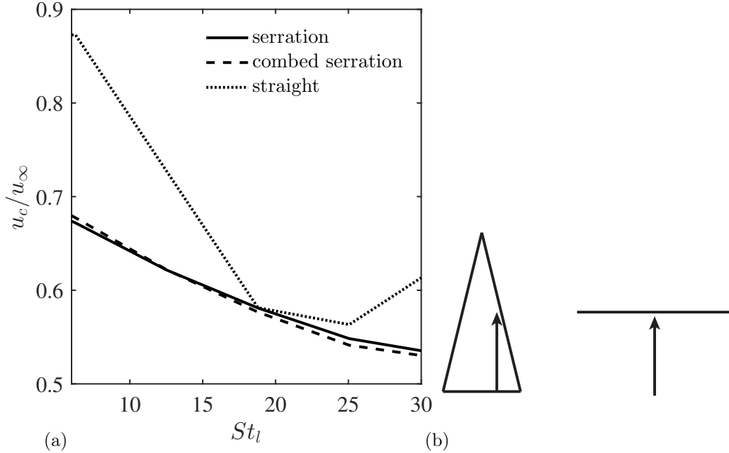
Figure 10. (a) Convective velocity ( u_c ) versus the Strouhal number based on the chord ( St_l ). (b) Sketch representative of the points used to compute the phase angle in the streamwise direction.
