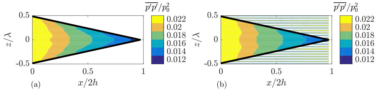
Figure 7. Intensity of the mean surface pressure fluctuation ( \overline{p'p'}/p_0^2 ): (a) serration and (b) combed serration. The serration edge in the x-z plane is indicated by means of continuous black lines.
