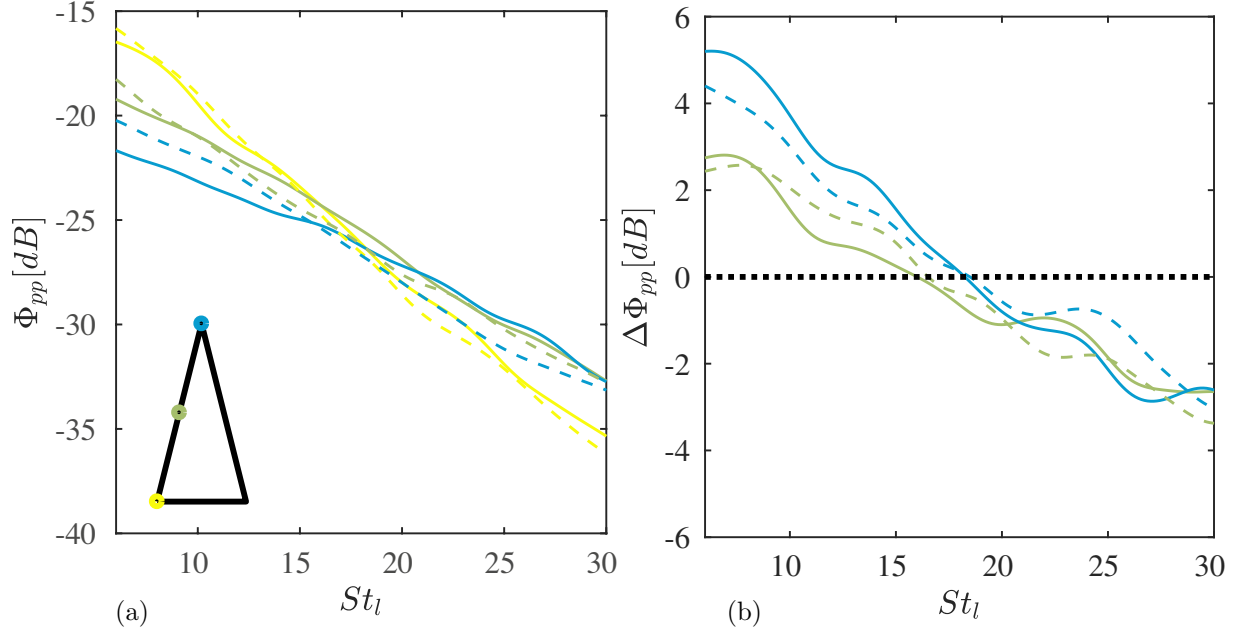
Figure 8. (a) Spectra of the surface pressure fluctuations ( \Phi_{pp} ) at three streamwise locations corresponding to x/2h = 0 (yellow), 0.5 (green) and 1 (blue). The continuous and dashed lines represent the serration and combed serration respectively. (b) \Delta\Phi_{pp} = \Phi_{pp}^{root} - \Phi_{pp}^{stream} with respect to the root location.
