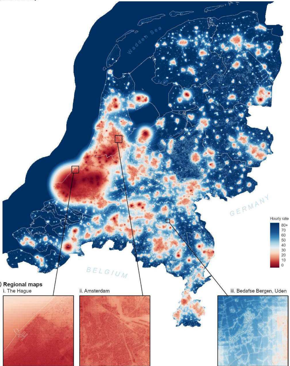
Figure 1 – Forecast map of Hourly Rates for the 2023 Perseids meteor shower. (a) The main map is valid for the near moonless night of August 13 at 04:00 UT (06:00 LT), assuming a radiant elevation of h=65^\circ , r=2.2 , ZHR=100 . (b) Local maps of Hourly Rates for (i.) The Hague, with HR=16 at the beach with the lowest sky brightness and best unobstructed view; (ii.) Amsterdam, with HR=18 at the Vondel Park; and (iii.) Bedafse Bergen near Uden
