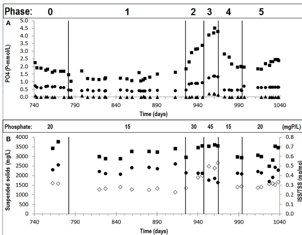
FIGURE 1 | Concentrations observed in the different cycles of the experimental phases studied: (A) orthophosphate concentrations in the influent (●), end of the anaerobic phase (■), and end of the aerobic phase (▲); and, (B) TSS concentrations in the end of the aerobic phase (■), VSS concentrations in the end of the aerobic phase (●) and ISS/TSS ratios (◇).
