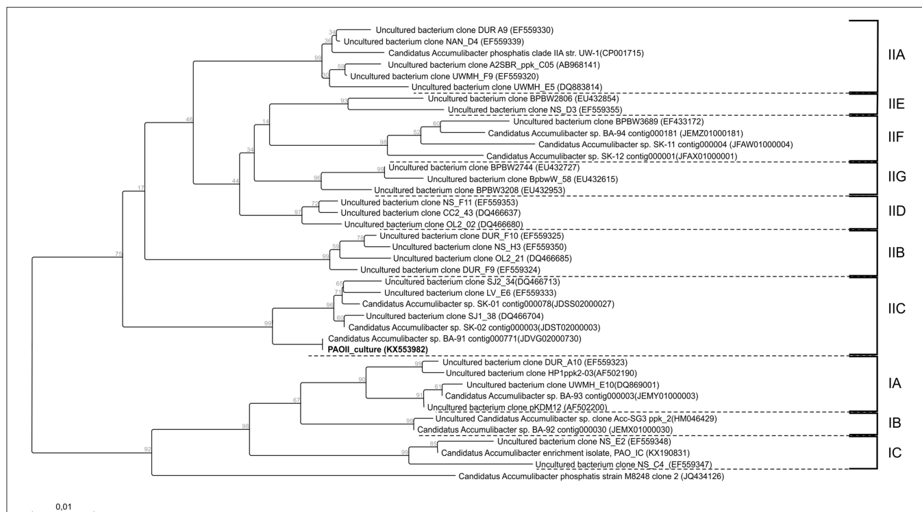
FIGURE 4 | Phylogenetic tree constructed using the neighbor joining method implemented in the CLC genomic workbench v7.5.1 package. The distance between sequences were measured using the kimura model. 332 amino-acid positions were used for calculation which corresponds to a near complete ppk1 gene. The sequence of the ppk1 gene from Rhodocyclus tenuis (AF502199) was used as an outgroup and afterwards pruned from the tree. Also bootstrap (1000 rounds) was performed and the resulting values were displayed on the branching points. All clades are indicated by the text IA till IC and IIA till IIG. The scale bar represent one percent difference in amino-acid composition. The sequence obtained in this study is indicated in bold.
