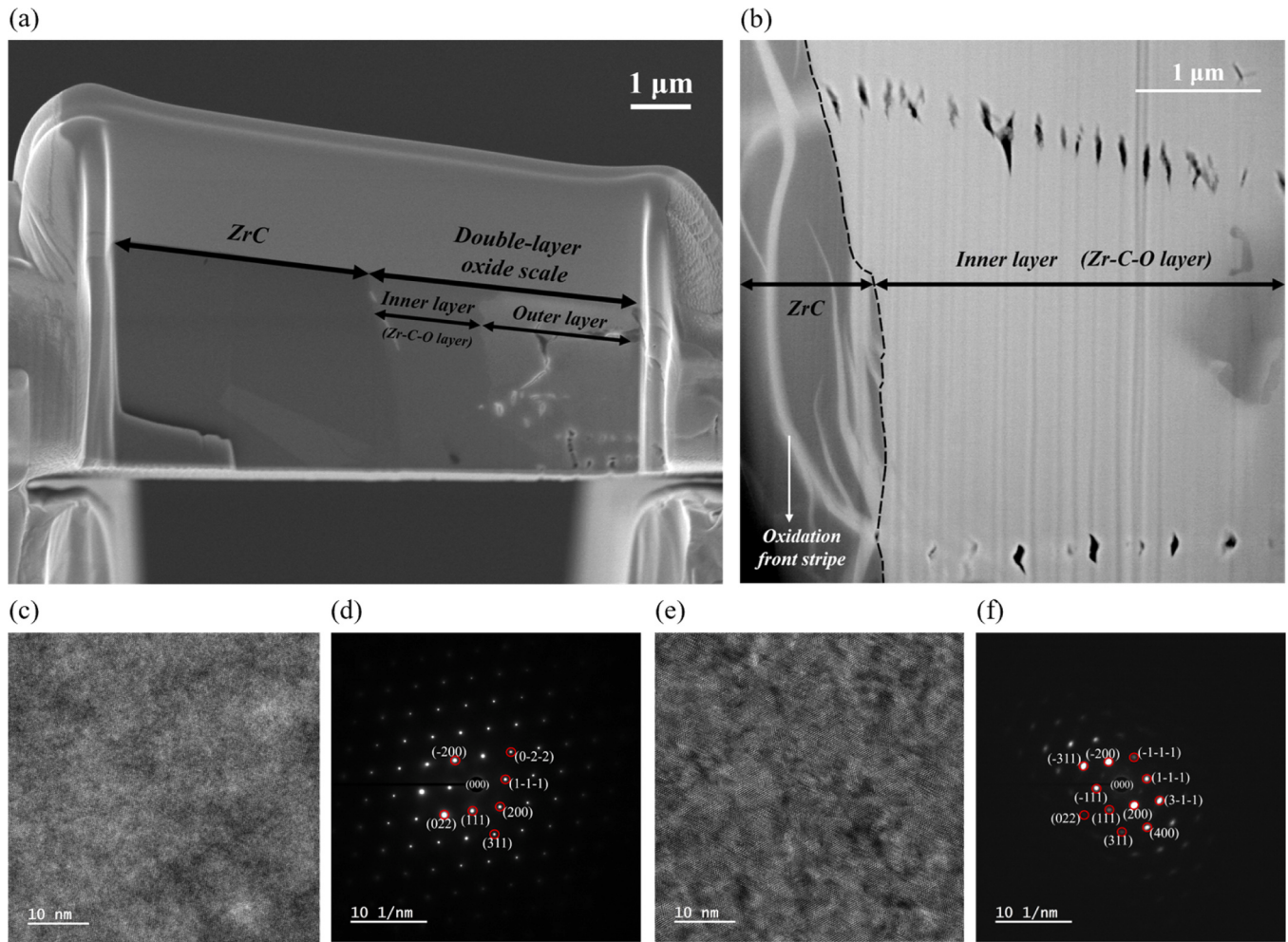
Fig. 1. (a) SEM image of the oxidized ZrC lamella (oxidation conditions: 600 °C; 2 % O 2 ; 10800 s). The double-layer oxide scale on ZrC substrate is demonstrated in the image. (b) STEM image HAADF mode of the oxidized ZrC lamella (600 °C; 2 % O 2 ; 10800 s) at the ZrC substrate/Zr–C–O layer interface, revealing the compact Zr–C–O layer, the oxidation front stripes, and the submicropores along the oxidation front stripe patterns. The black dashed line is the interface of ZrC substrate and Zr–C–O layer. (c) HRTEM image of ZrC substrate of the lamella in (a). (d) Selected area electron diffraction pattern (SAEDP) of ZrC substrate of the lamella in (a) with zone axis: [01–1]. The interplanar spacings ( d_{hkl} ) are approximately: 2.72 Å for d_{111} , 2.36 Å for d_{200} , 1.66 Å for d_{220} , and 1.42 Å for d_{311} , which are consistent with the face-centered cubic crystal structure of ZrC. (e) HRTEM image of outer-layer oxide scale of the lamella in (a). (f) SAEDP of outer-layer oxide scale of the lamella in (a) with zone axis: [01–1]. The interplanar spacings ( d_{hkl} ) are approximately: 2.94 Å for d_{111} , 2.55 Å for d_{200} , 1.80 Å for d_{220} , 1.54 Å for d_{311} , and 1.27 Å for d_{400} , which are consistent with the cubic crystal structure of ZrO 2 (c-ZrO 2 ).
