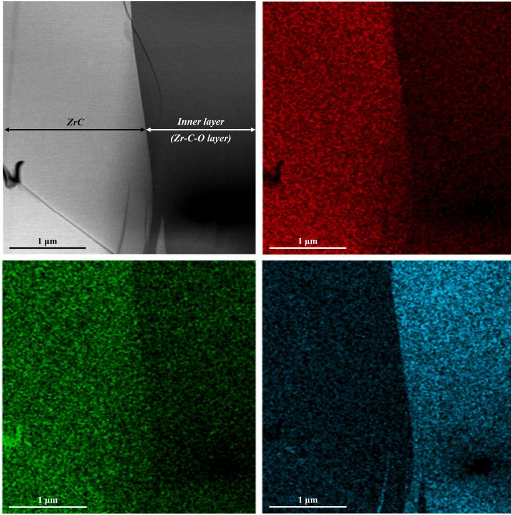
Fig. 4. HRTEM-EDX elemental mapping at the ZrC substrate/Zr-C-O layer interface. Zr distribution is shown in red, C in green, and O in blue.
