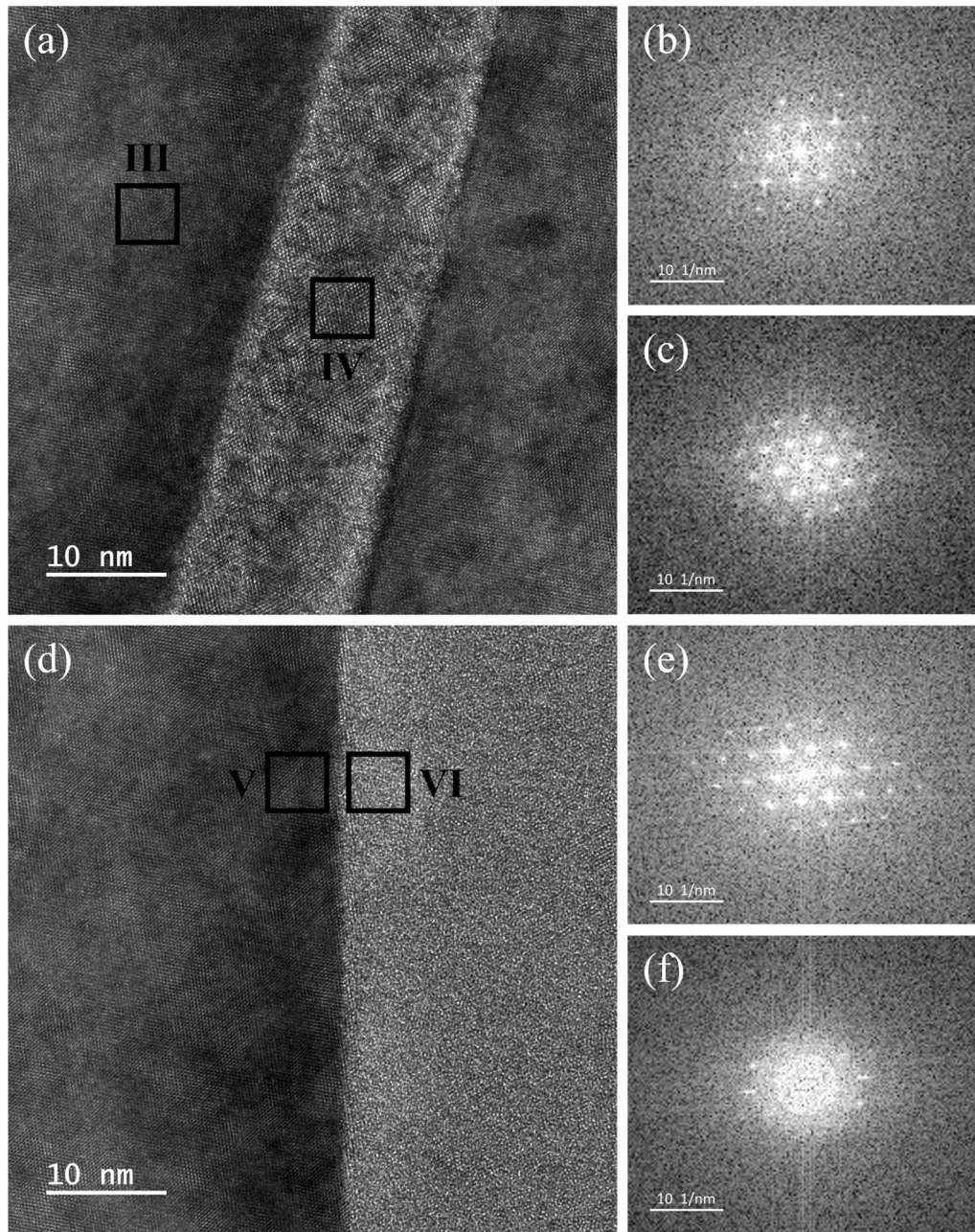
Fig. 3. (a) HRTEM image at the oxidation front stripe with zone axis: [01-1] . The oxidation front stripe is shown in the middle bright region. The location of the HRTEM image is Square I in Fig. 2(a). (b) Cubic FFT pattern of ZrC substrate located at Square III in (a). (c) Cubic FFT pattern of oxidation front stripe located at Square IV in (a). (d) HRTEM image at the interface of ZrC (left side) and the Zr-C-O layer (right side) with zone axis: [01-1] . The location of the HRTEM image is Square II in Fig. 2(a). (e) Cubic FFT pattern of ZrC substrate located at Square V in (d). (f) FFT pattern of Zr-C-O layer located at Square VI in (d).
