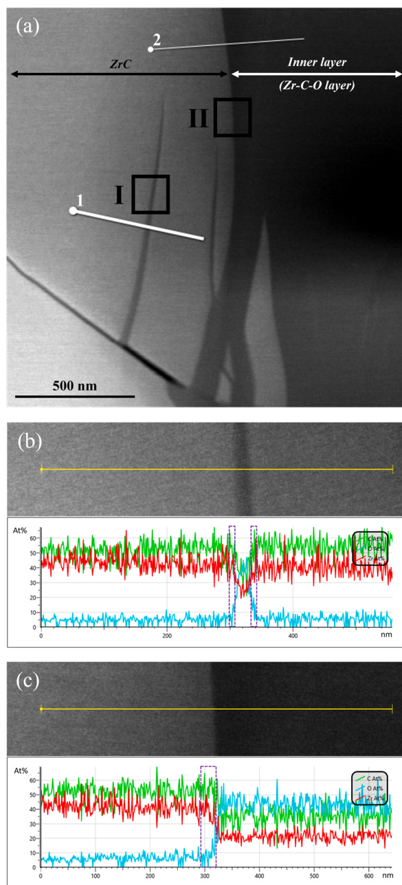
Fig. 2. (a) TEM image at the interface of ZrC substrate and Zr–C–O layer. Line 1 is the HRTEM-EDX line analysis location of (b), and Line 2 is the HRTEM-EDX line analysis location of (c). Square I is the HRTEM image location of the oxidation front stripe (Fig. 3(a)). Square II is the HRTEM image location of the ZrC/Zr–C–O layer interface (Fig. 3(d)). (b) HRTEM-EDX line analysis of Line 1 in (a). (c) HRTEM-EDX line analysis of Line 2 in (a). The purple dashed square regions indicate the onset of the increase in O at% up to the point near its saturation, which reflects the O/Zr atomic percent ratio < 2.
