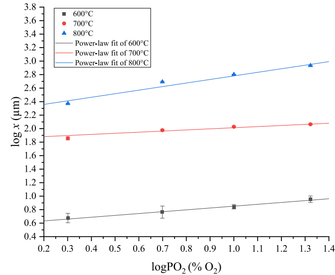
Fig. 7. Log-log plot of outer-layer oxide scale thickness ( x ) versus oxygen partial pressure (PO 2 ) at 600 °C (black), 700 °C (red), and 800 °C (blue). Symbols represent experimental data with error bars indicating standard deviations transformed into log space. Solid lines correspond to power-law fits, which appear linear on the log-log scale.
