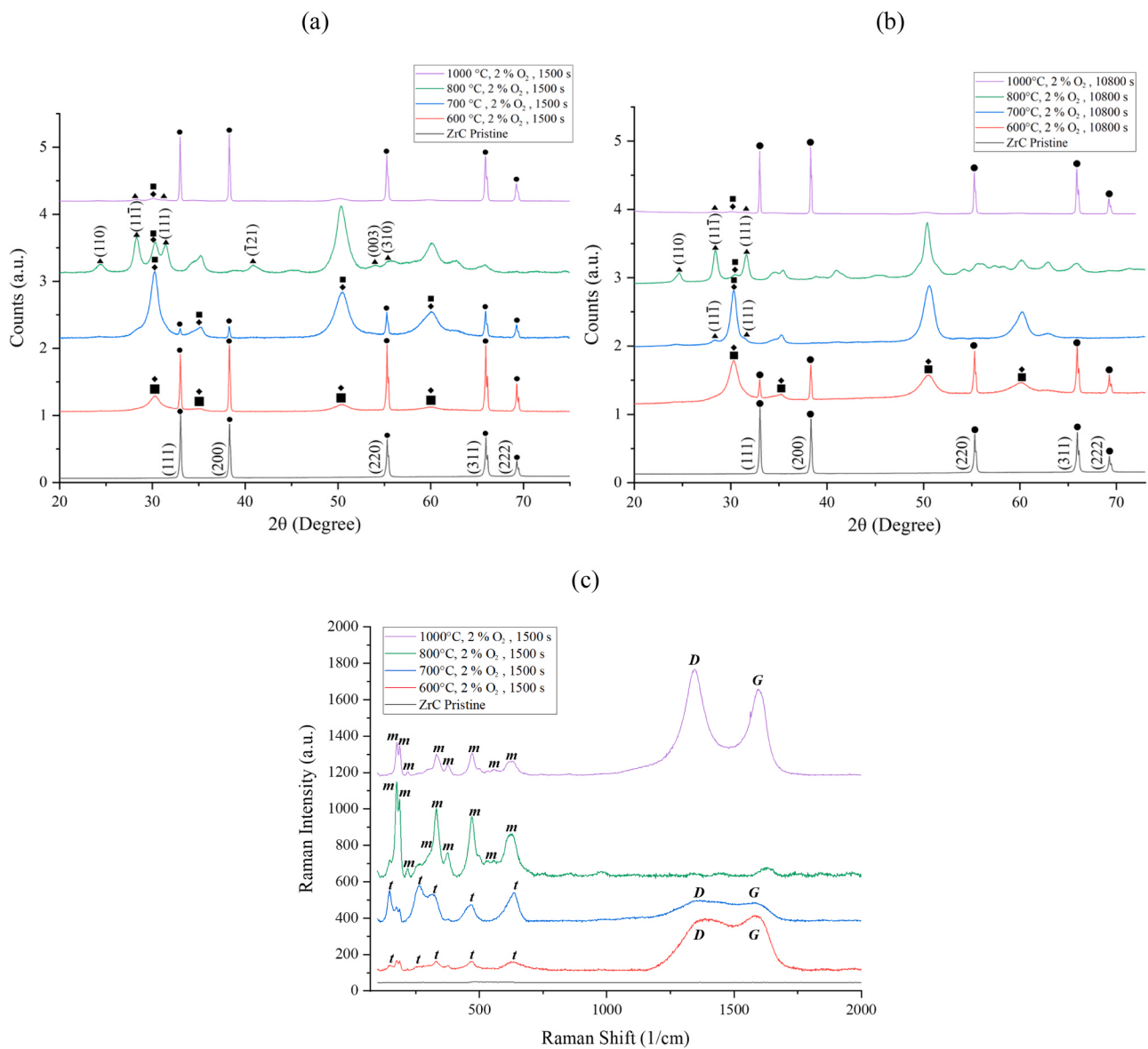
Fig. 5. (a)(b) XRD patterns of temperature dependent oxidation. (a) Oxidation duration: 1500 s. (b) Oxidation duration: 10800 s. ●: ZrC; ■: c-ZrO 2 ; ◆: t-ZrO 2 ; ▲: m-ZrO 2 . (c) Raman spectra of temperature dependent oxidation. t: t-ZrO 2 ; m: m-ZrO 2 ; D: D-band of free carbon; G: G-band of free carbon. t-ZrO 2 Raman peaks: 150, 272, 315, 462, 642 cm -1 . m-ZrO 2 Raman peaks: 179, 188, 222, 307, 334, 344, 381, 480, 557, 617, 632 cm -1 . Raman peaks of carbon: D-band at 1350 cm -1 , and G-band at 1580 cm -1 .
