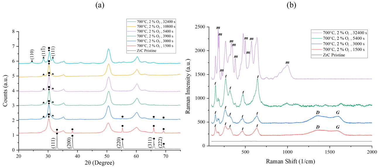
Fig. 6. (a) XRD patterns of time dependent oxidation at 700 °C; 2 % O 2 . ●: ZrC; ■: c-ZrO 2 ; ◆: t-ZrO 2 ; ▲: m-ZrO 2 . (b) Raman spectra of time dependent oxidation at 700 °C; 2 % O 2 . t: t-ZrO 2 ; m: m-ZrO 2 ; D: D-band; G: G-band of free carbon.
