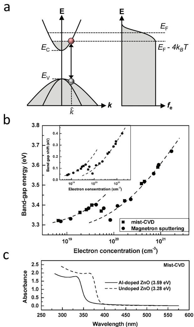
Figure 12. a) Principle of Burstein–Moss shift, left panel: Schematic band structure with filled electron states shown in grey. \hat{k} represents the k -vector for the optical absorption process lowest in photon energy. Right panel: Electron distribution function for a degenerate electron gas with the Fermi level in the conduction band (Redrawn from ref. [1]). b) Apparent “bandgap” energy as a function of electron concentration in AZO. The inset shows the apparent “bandgap” shift as a function of electron concentration (Reproduced with permission. [69] Copyright 2007, AIP Publishing). c) Comparison of the absorption spectrum of Al-doped (AZO) and undoped ZnO thin films (Adapted with permission. [69] Copyright 2007, AIP Publishing).
