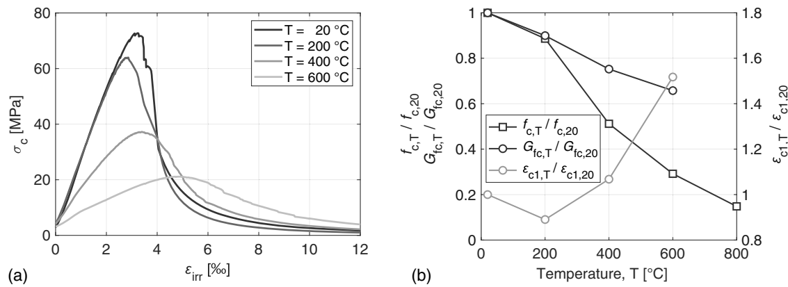
Fig. 7. (a) Average compressive stress-strain curves; and (b) evolution of nominal compressive peak strength, specific compressive fracture energy, and strain at peak stress, after cooling.
