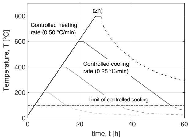
Fig. 1. Temperature cycles at 200°C, 400°C, 600°C, and 800°C.
