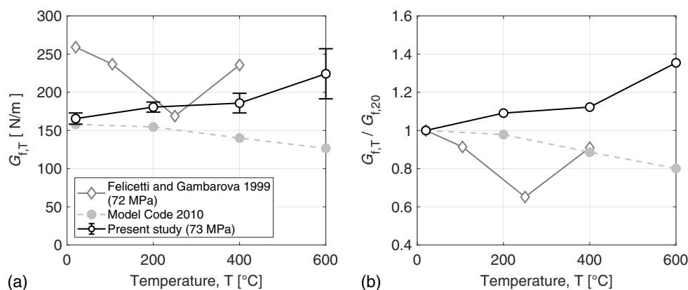
Fig. 16. Evolution of (a) total; and (b) relative specific tensile fracture energy after cooling.
