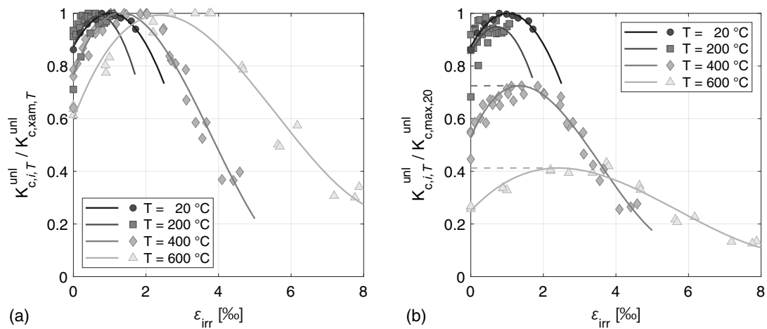
Fig. 10. Evolution of (a) mechanical; and (b) total unloading stiffness in compression.
