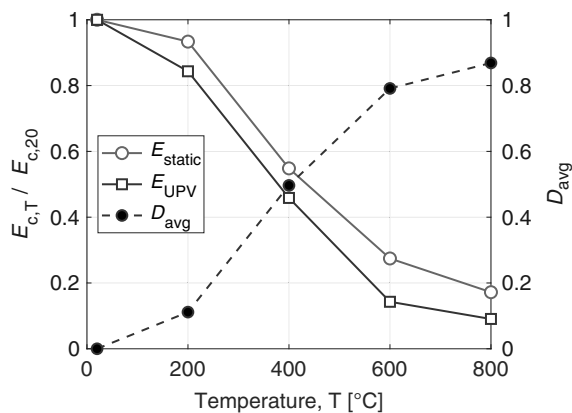
Fig. 5. Relative modulus of elasticity and damage for different temperatures after cooling.
