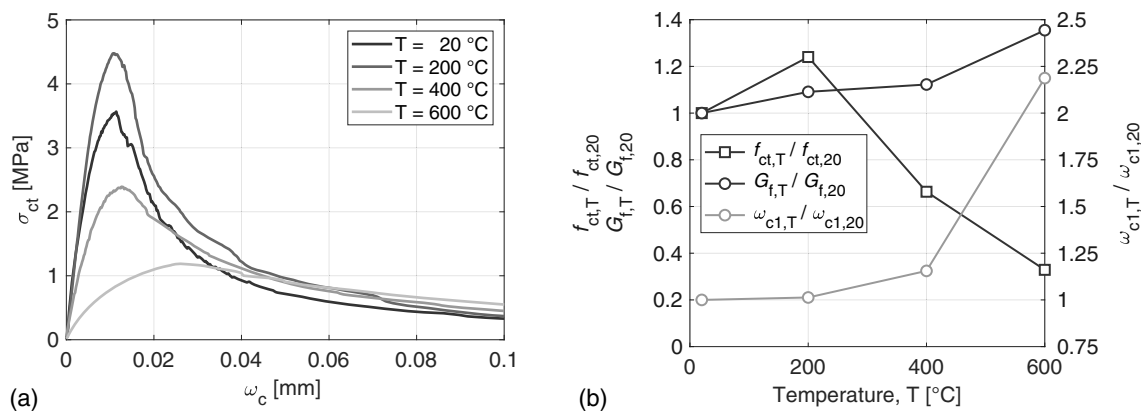
Fig. 9. (a) Average tensile stress-crack opening curves; and (b) evolution of tensile nominal peak strength, specific tensile fracture energy, and crack opening at peak stress after cooling.
