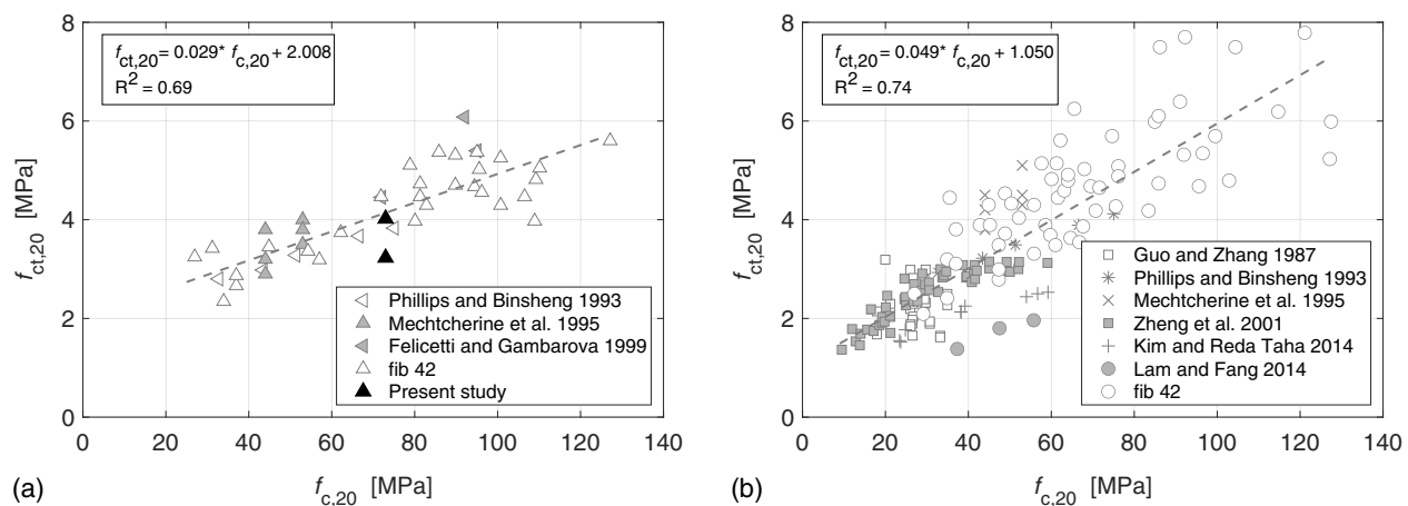
Fig. 14. Scatter of uniaxial tensile tests at 20°C on (a) notched; and (b) unnotched specimens characterized by different concrete strength.
