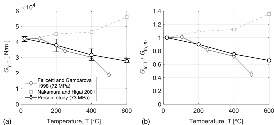
Fig. 17. Evolution of (a) total; and (b) relative specific compressive fracture energy after cooling.
