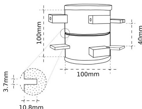
Fig. 4. Instrumentation for uniaxial tensile tests.
