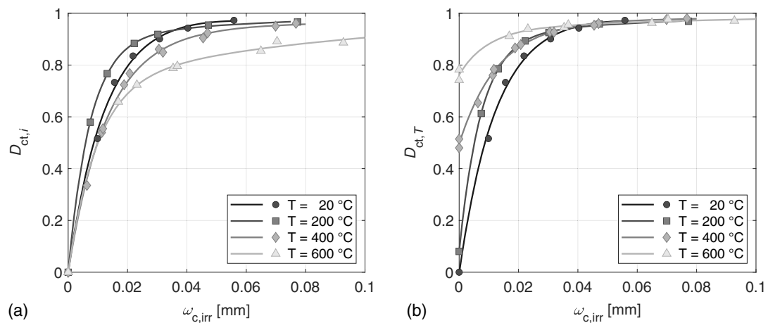
Fig. 11. Evolution of (a) mechanical ( D_{ct,i} ); and (b) total ( D_{ct,T} ) internal damage in tension.
