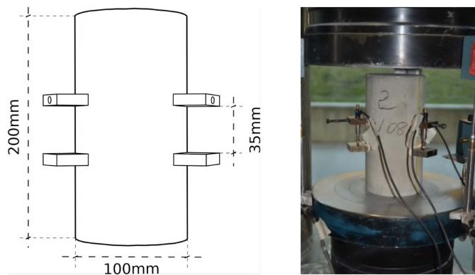
Fig. 3. Instrumentation for modulus of elasticity tests.
