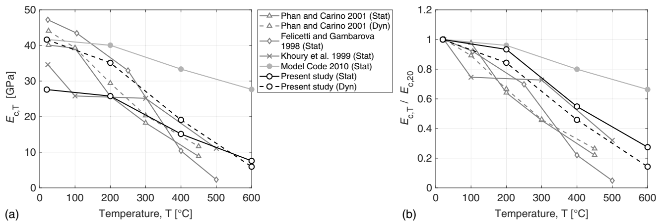
Fig. 12. Experimental results of (a) total; and (b) relative modulus of elasticity after cooling.
