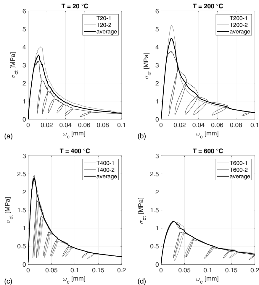
Fig. 8. Tensile nominal stress-crack opening curves for different temperatures after cooling.
