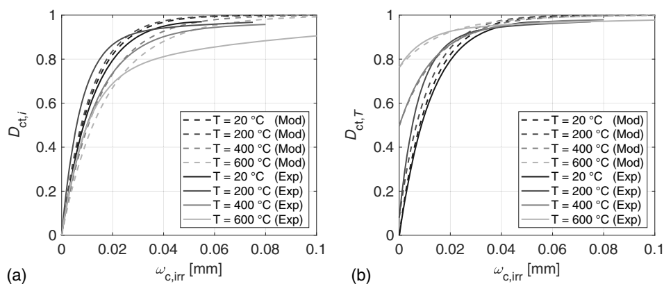
Fig. 18. Comparison of (a) mechanical; and (b) total damage evolution between Nechnech et al. (2002) model (Mod) and the obtained experimental results (Exp).
