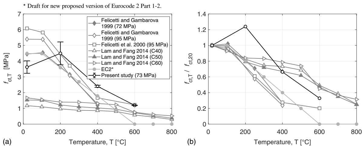
Fig. 15. Experimental results of (a) total; and (b) relative tensile strength after cooling.
