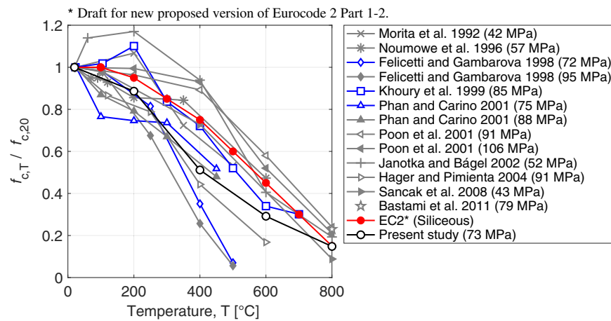
Fig. 13. Experimental results of relative compressive strength at different temperatures after cooling.
