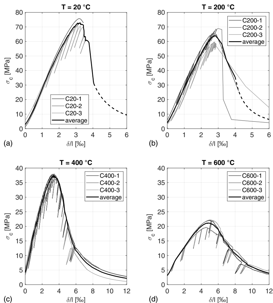
Fig. 6. Compressive nominal stress-strain curves for different temperatures after cooling.
