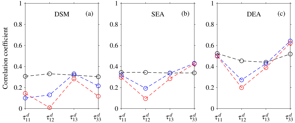
Figure 1: Correlation coefficients for the normal and cross terms of the modeled and the actual deviatoric part of the SGS stress tensor. Isotropic ( -\circ- ); weak rotation ( -\circ- ); strong rotation ( -\circ- ).
