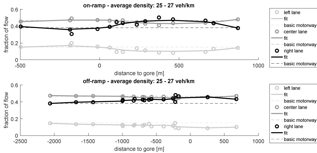
Figure 3.9. Lane flow distribution at ramps with low density.
