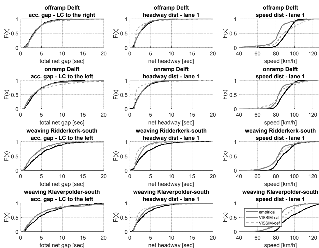
Figure 6.5. Calibration results.
