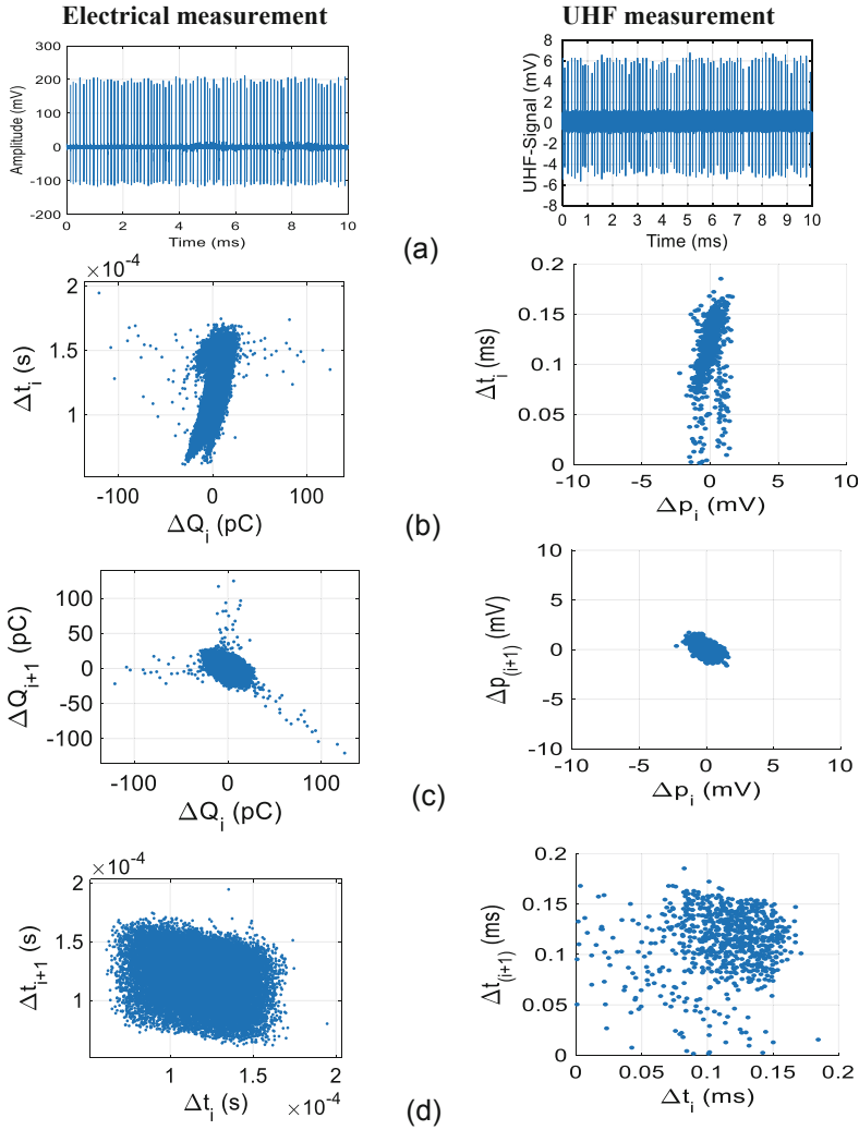
Fig. 4. PSA patterns of configuration I, showing (a) discharge pulse stream, plot of (b) \Delta Q vs. \Delta t (c) \Delta Q_i vs. \Delta Q_{i+1} (d) \Delta t_i vs. \Delta t_{i+1} .
