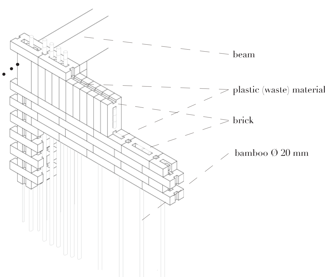
facade
