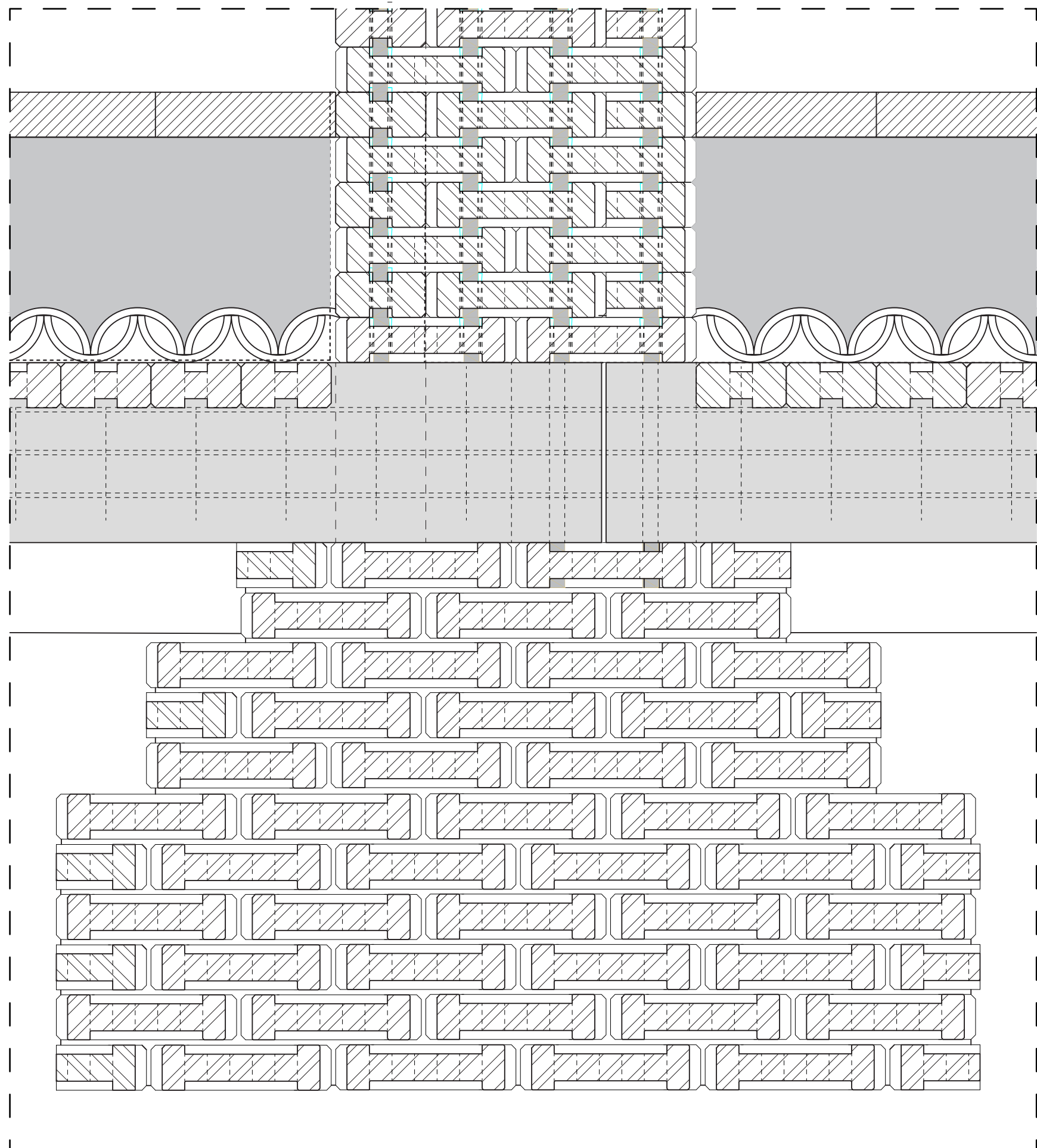
detail C foundation year 5 1:5
