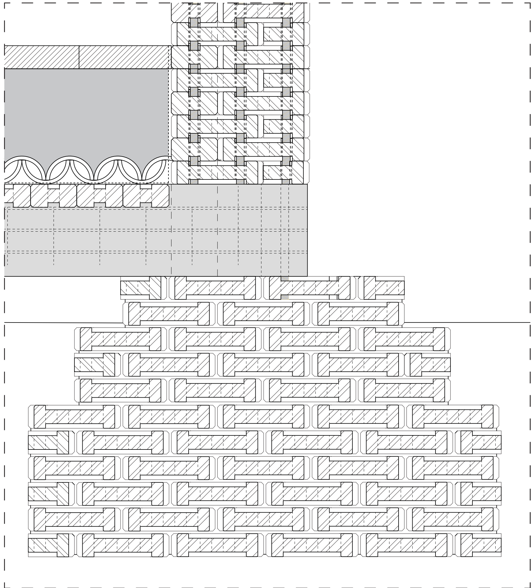
detail C foundation year 0 1:5
