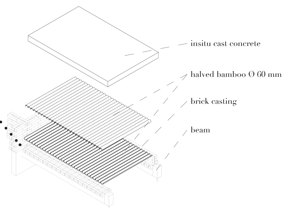
floor/roof
