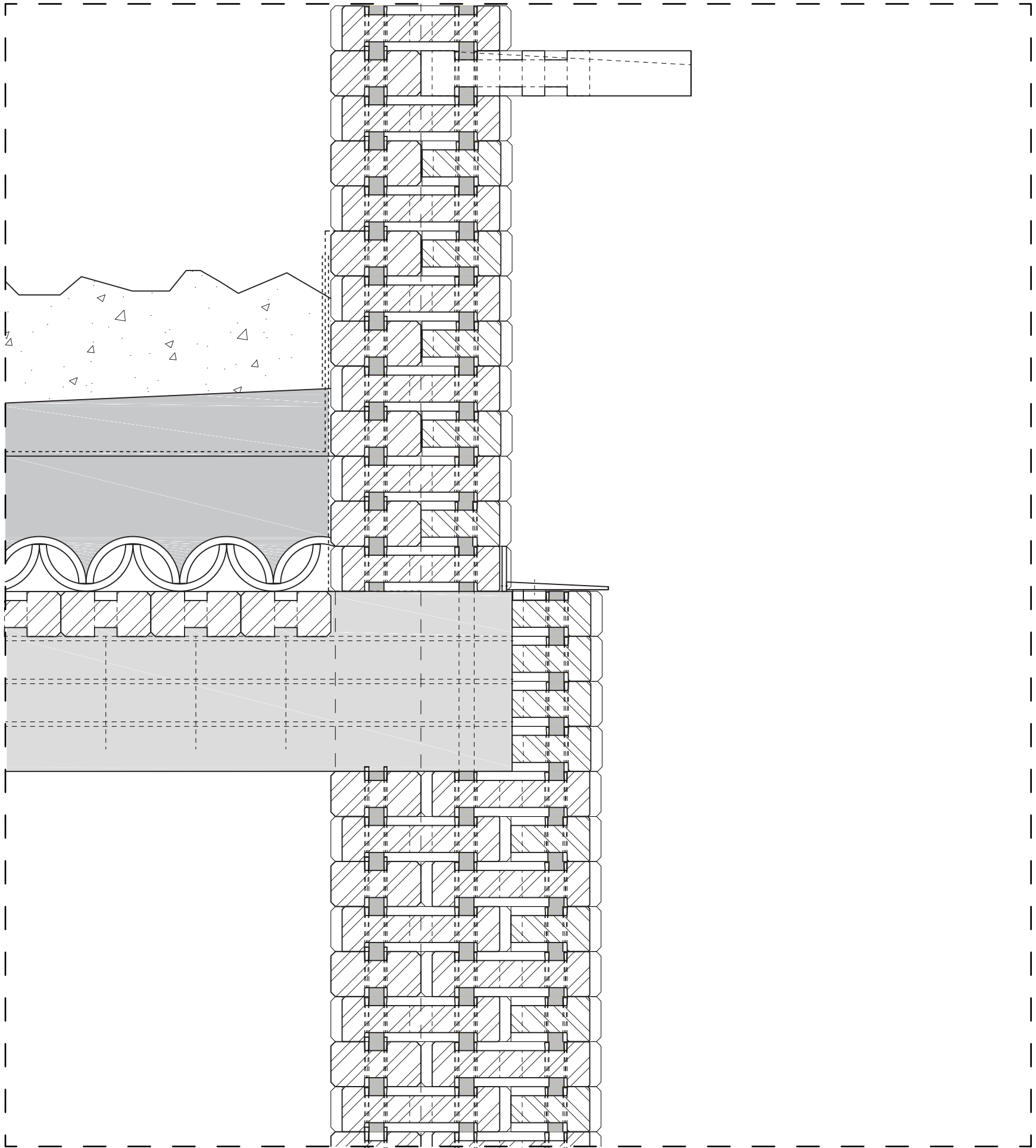
detail B roof/floor year 0 1:5
