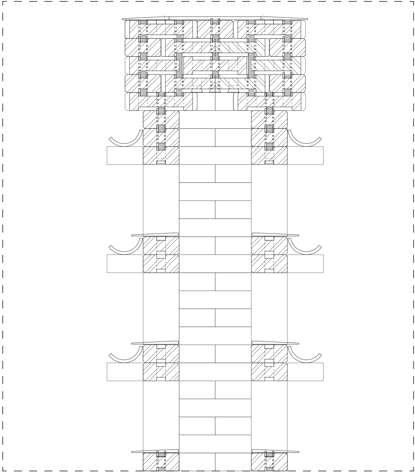
detail A chimney 1:5
