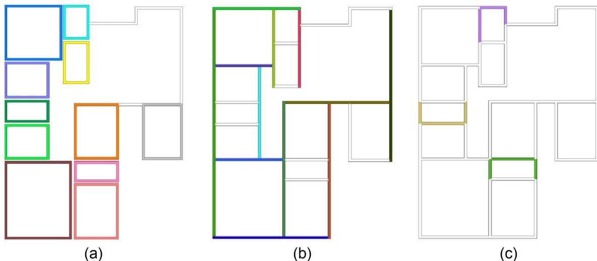
Fig. 18. (a) Fully volumetric solution (11VM); (b) fully panelized solution (0VM); and (c) three-VM solution.
