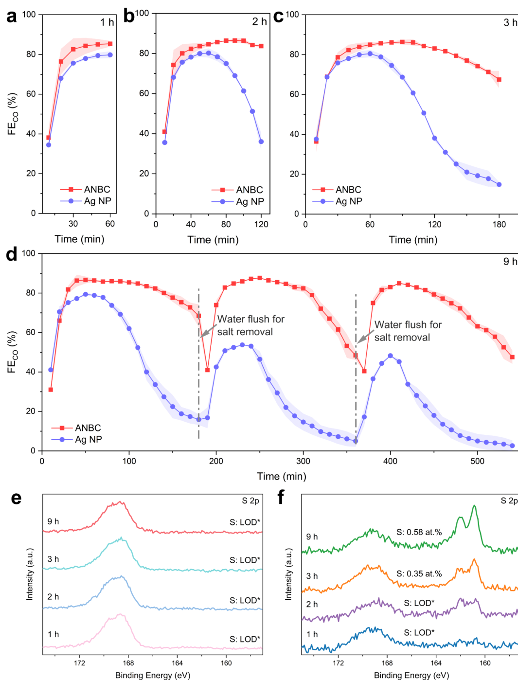
Figure 8. High current density CO 2 electrolysis tests of ANBC and Ag NP catalysts conducted in an MEA reactor in the presence of 100 ppm of SO 2 . FE CO of ANBC and Ag NP catalysts with reaction duration of (a) 1 h, (b) 2 h, (c) 3 h, and (d) 9 h. High-resolution S 2p XPS spectra of (e) ANBC and (f) Ag NP gas diffusion electrodes after different electrolysis durations.
