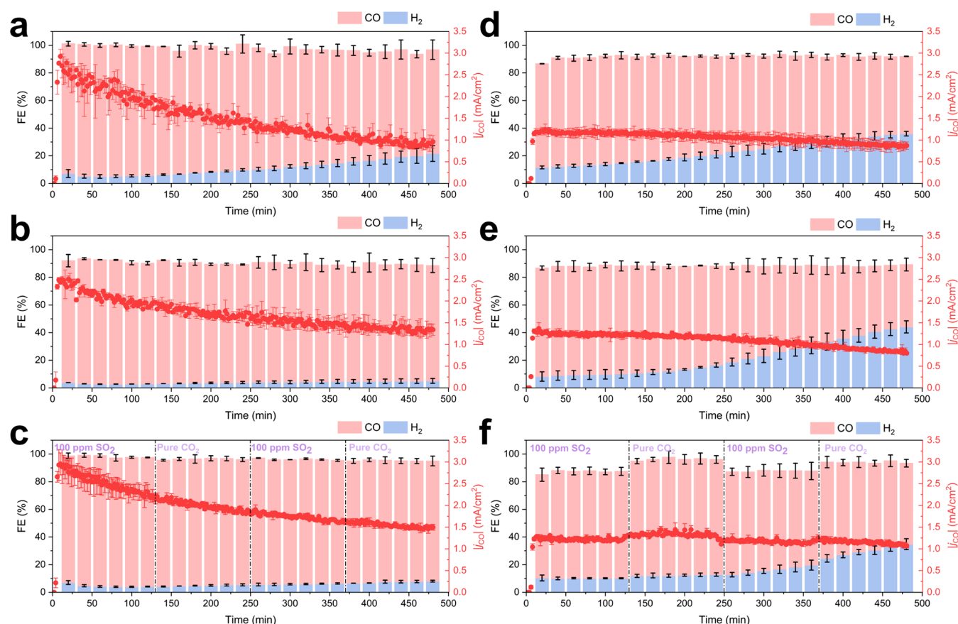
Figure 5. Longer-term \text{CO}_2 reduction performance tests. Faradaic efficiencies and j_{\text{CO}} during 8-h stability tests for (a) ANBC and (d) Ag foil electrodes at -1.0 V vs RHE in a \text{CO}_2 -saturated 0.1 M \text{KHCO}_3 electrolyte. Faradaic efficiencies and j_{\text{CO}} during 8-h stability tests for (b) ANBC and (e) Ag foil electrodes at -1.0 V vs RHE in a \text{CO}_2 + 100 ppm of \text{SO}_2 gas mixture saturated 0.1 M \text{KHCO}_3 electrolyte. Faradaic efficiencies and j_{\text{CO}} of \text{CO}_2 + 100 ppm of \text{SO}_2 and pure \text{CO}_2 electrolysis over (c) ANBC and (f) electrode at -1.0 V vs RHE in 0.1 M \text{KHCO}_3 electrolyte over 8 h, the gas feed is modulated every 2 h.
