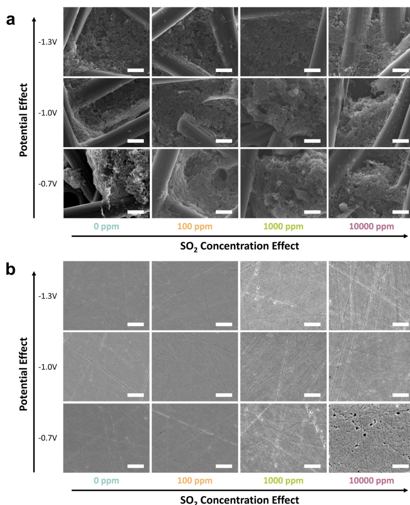
Figure 6. Surface characterization of ANBC and silver electrodes after electrolysis. SEM images of (a) ANBC (scale bar: 5 \mu\text{m} ) and (b) Ag foil (scale bar: 2.5 \mu\text{m} ) electrodes after 1 h electrolysis in the presence of different concentration of \text{SO}_2 impurities and different potentials.
