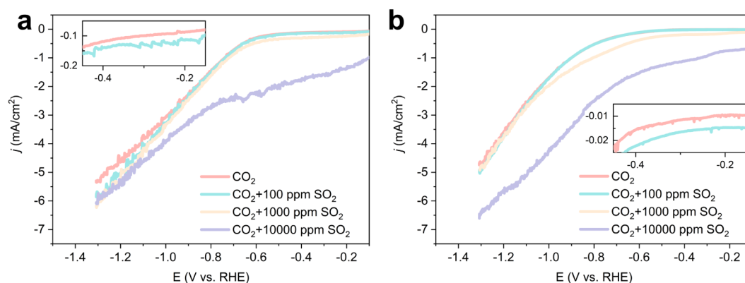
Figure 3. Voltammograms of ANBC and silver with varying \text{SO}_2 concentrations. LSV curves of (a) ANBC electrodes and (b) Ag foil electrodes, recorded in a 0.1 M \text{KHCO}_3 catholyte saturated with \text{CO}_2 , both without \text{SO}_2 and in the presence of varying concentrations of \text{SO}_2 impurities.
