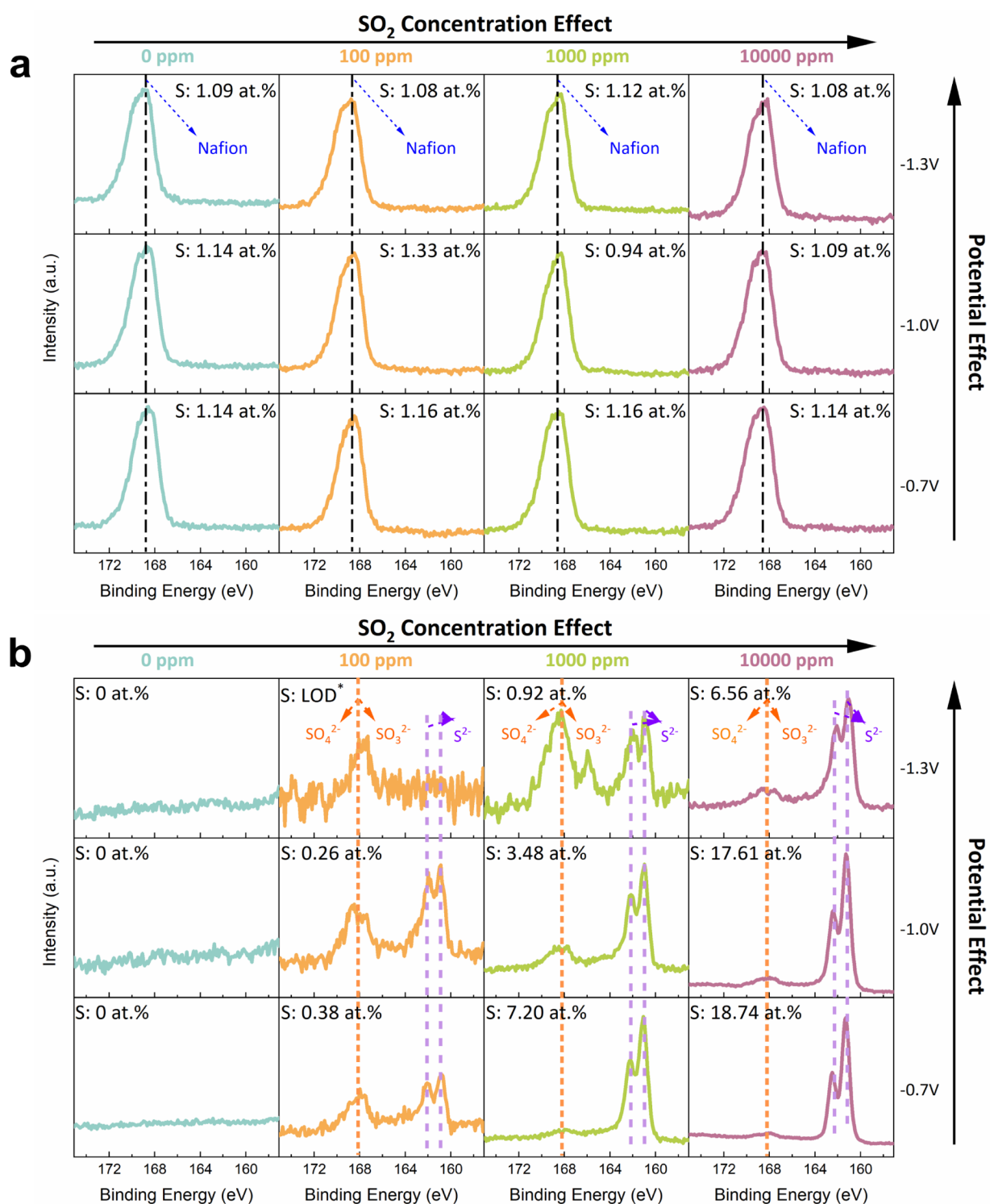
Figure 7. Characterization of the chemical composition of ANBC and silver electrodes after electrolysis. S 2p XPS spectrum of (a) ANBC and (b) Ag foil electrodes after 1 h electrolysis in the presence of different concentration of SO 2 impurities and different potentials. (*LOD = the limit of detection).
