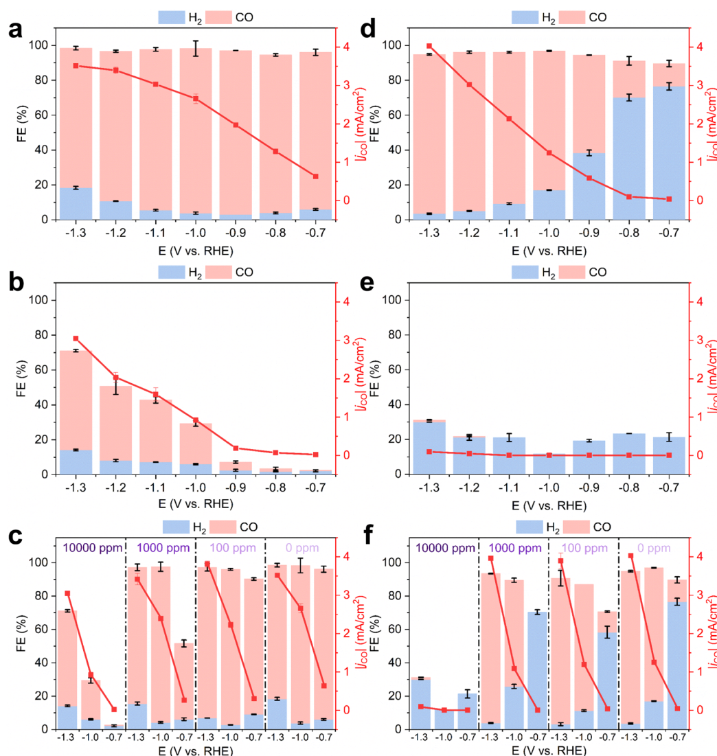
Figure 4. Electrochemical CO 2 reduction performance of ANBC and silver at varying SO 2 concentrations. Faradaic efficiencies and partial current densities for CO production on (a) ANBC and (d) Ag foil electrodes in a CO 2 -saturated 0.1 M KHCO 3 electrolyte with varying applied potentials, from −0.7 to −1.3 V vs RHE. Faradaic efficiencies and partial current densities for CO production on (b) ANBC and (e) Ag foil electrodes in the presence of 10,000 ppm of SO 2 impurity, from −0.7 to −1.3 V vs RHE. Faradaic efficiencies and partial current densities for CO production on (c) ANBC and (f) Ag foil electrodes with the presence of different concentrations of SO 2 impurities at −0.7, −1.0, and −1.3 V vs RHE.
