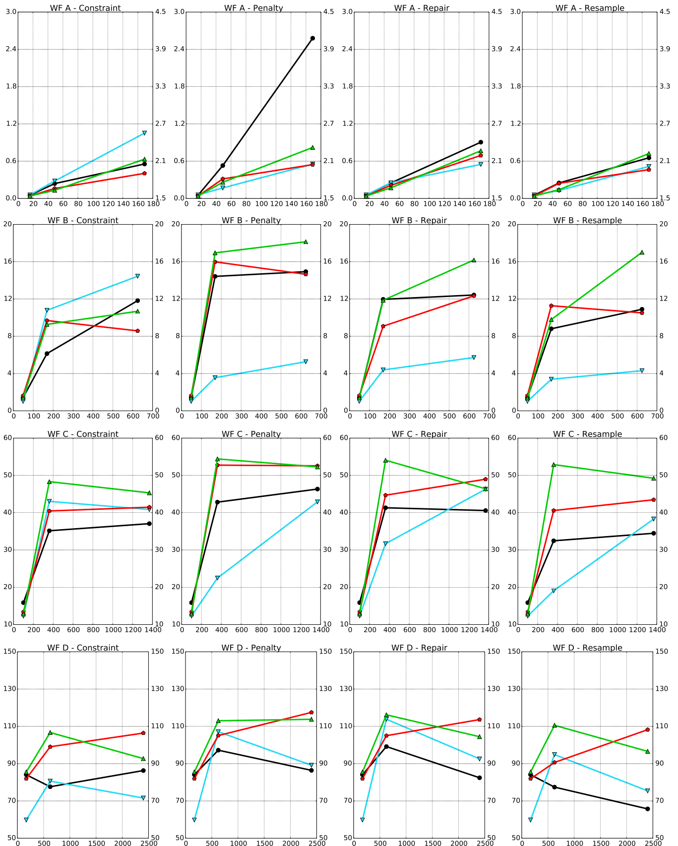
Fig. 15. Time needed by each optimization algorithm to converge for the different constraint handling techniques. The x-axis shows the number of variables and the y-axis displays the average time, in hours, needed for termination. MOGOMEA - red; o-MOGOMEA - green; NSGA-II - black; c-NSGA-II - blue. (For interpretation of the references to color in this figure legend, the reader is referred to the web version of this article.)
