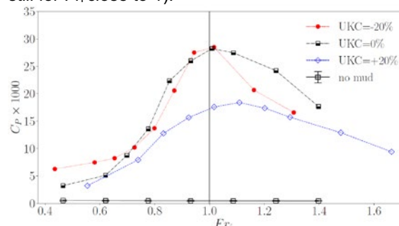
Figure 6 Pressure resistance coefficient versus densimetric Froude number for different UKCs.
