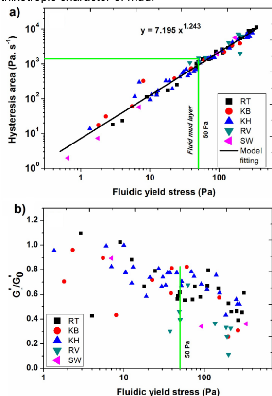
Figure 3 Hysteresis area (obtained from the thixotropy loop test) as a function of fluidic yield stress for different locations in the Port of Hamburg. (b) equilibrium structural parameter ( G'_{\infty}/G'_0 ) as a function of fluidic yield stress for different locations in the Port of Hamburg. Green solid line represents the critical value of fluidic yield stress (50 Pa) and hysteresis area ( 1400 \text{ Pa} \cdot \text{s}^{-1} ). Adapted from [9].
