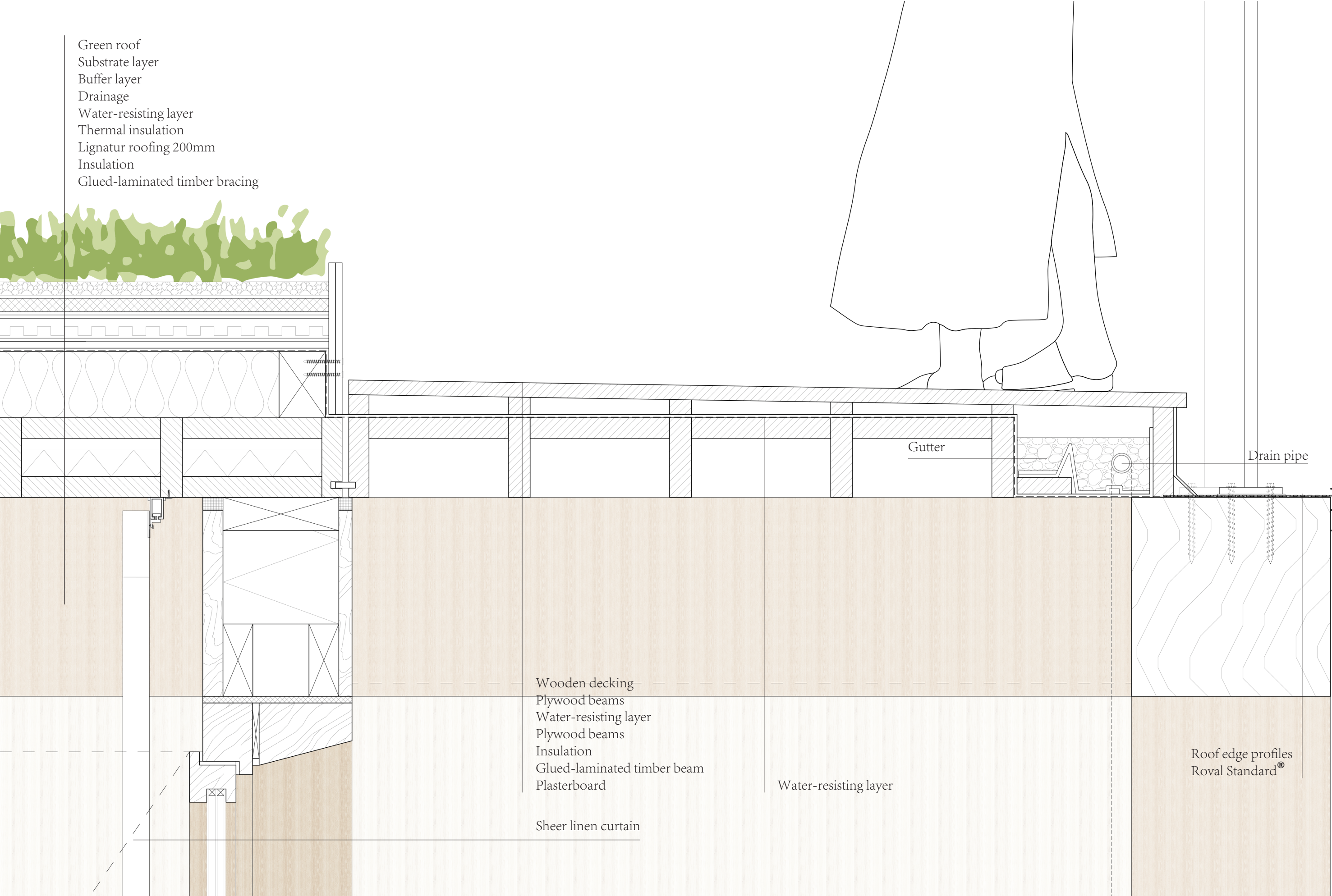
Detail 4 1:5
