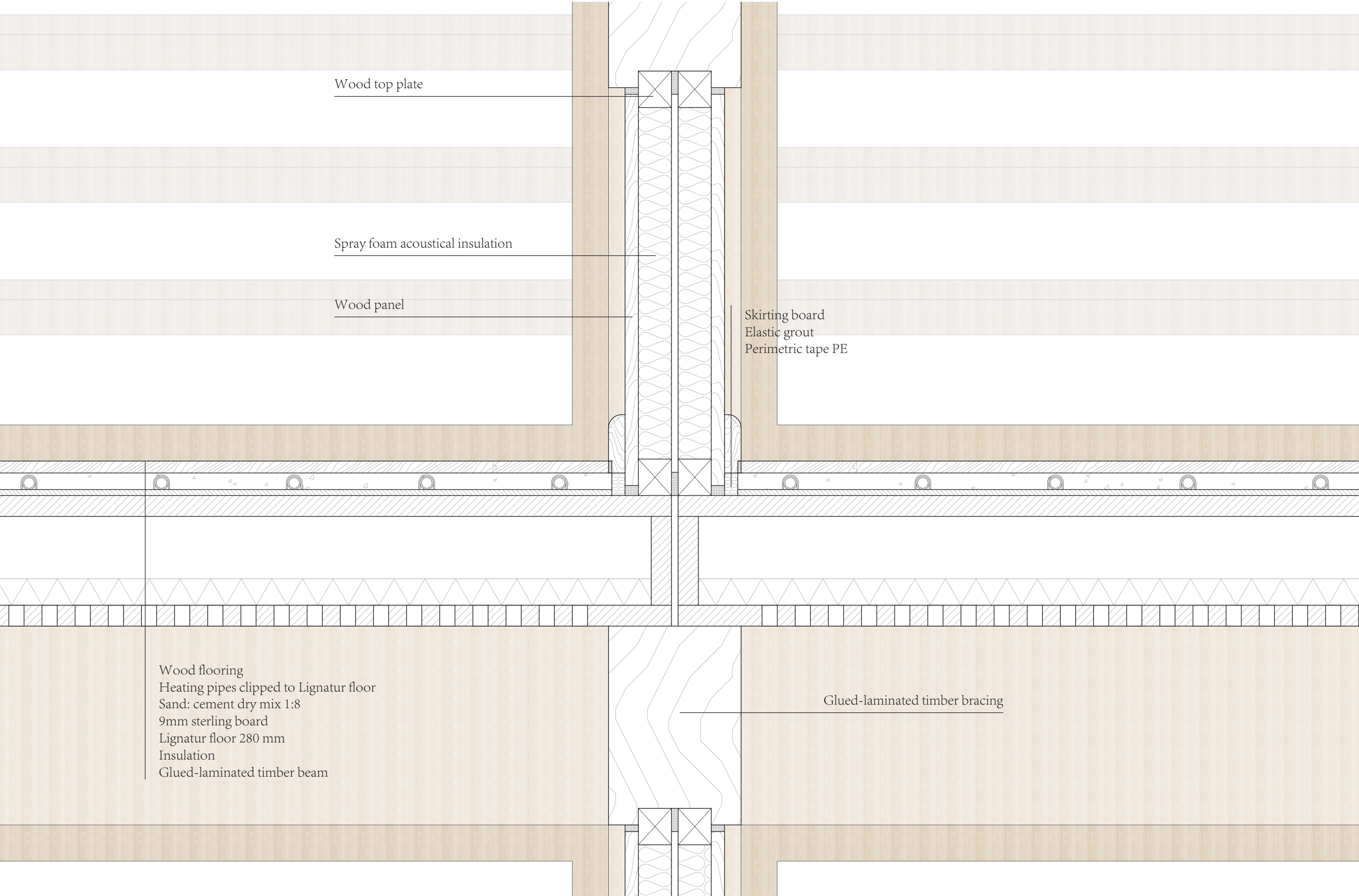
Detail 3 1:5
