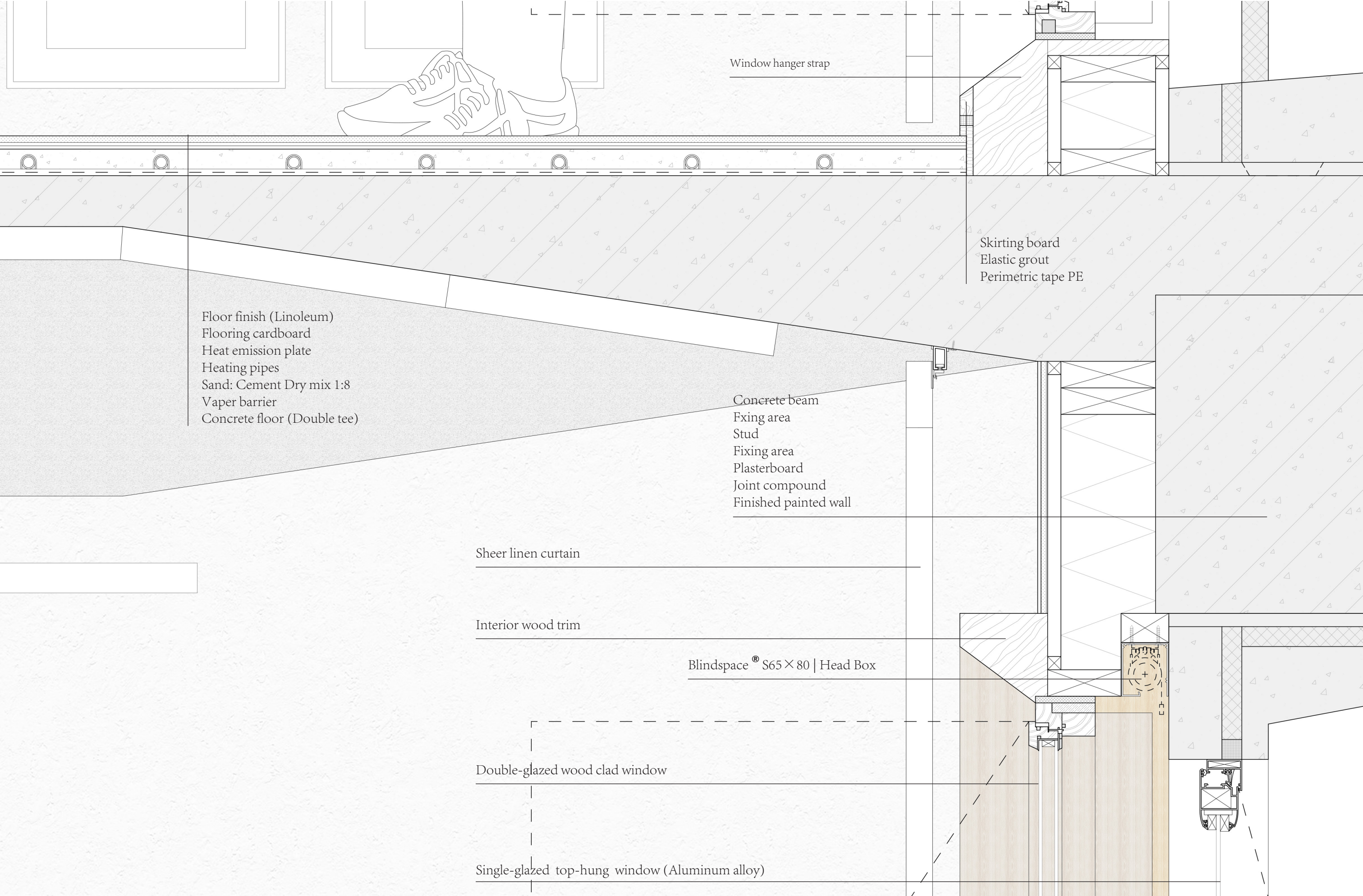
Detail 2 1:5
