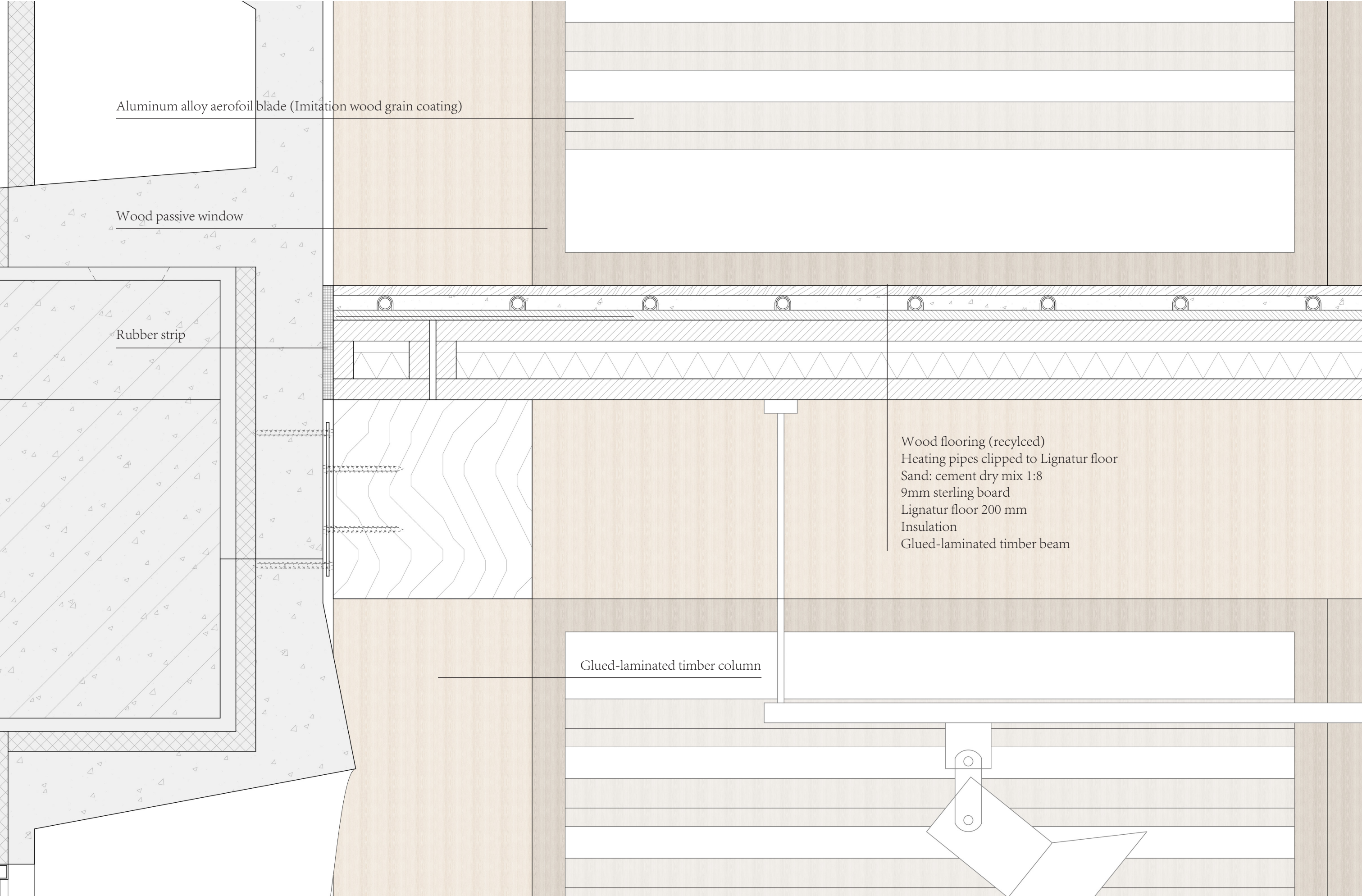
Detail 7 1:5
