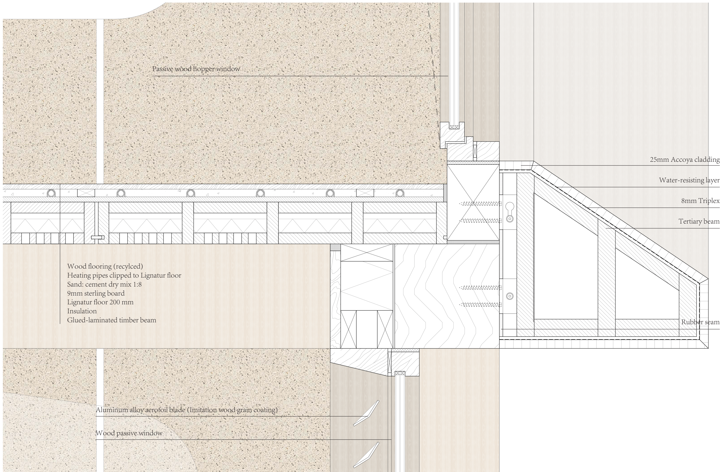
Detail 8 1:5
