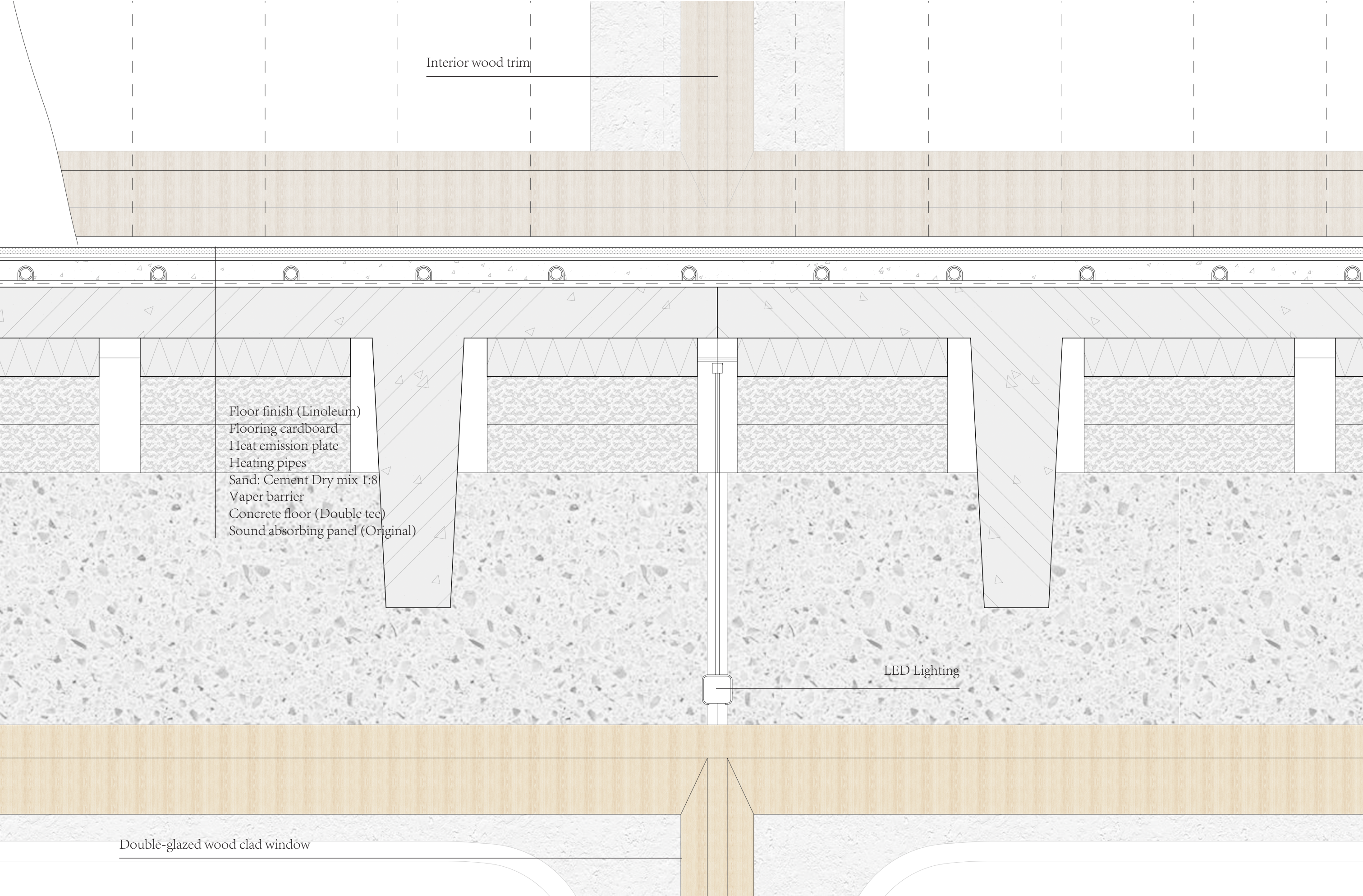
Detail 1 1:5
