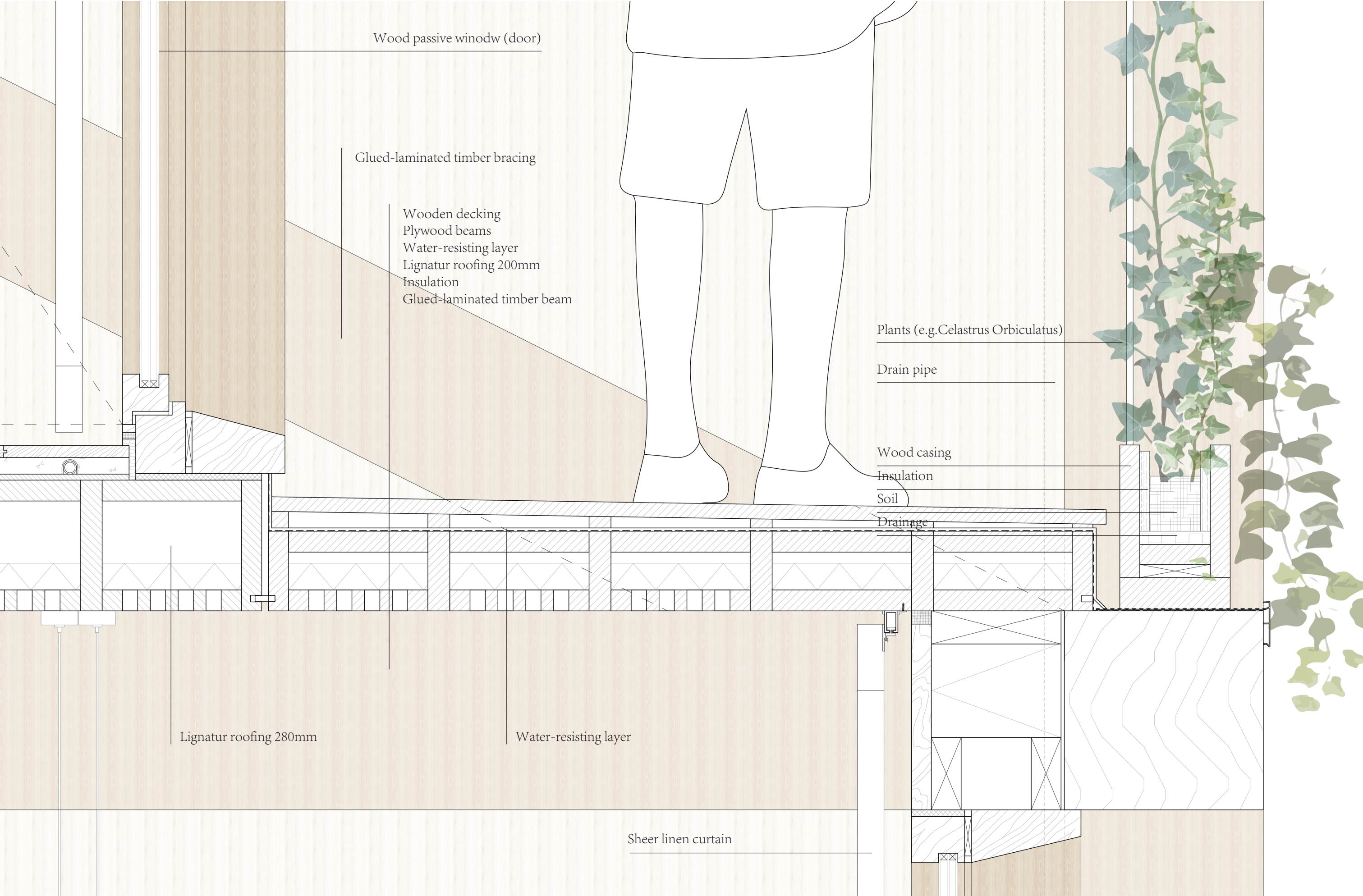
Detail 5 1:5
