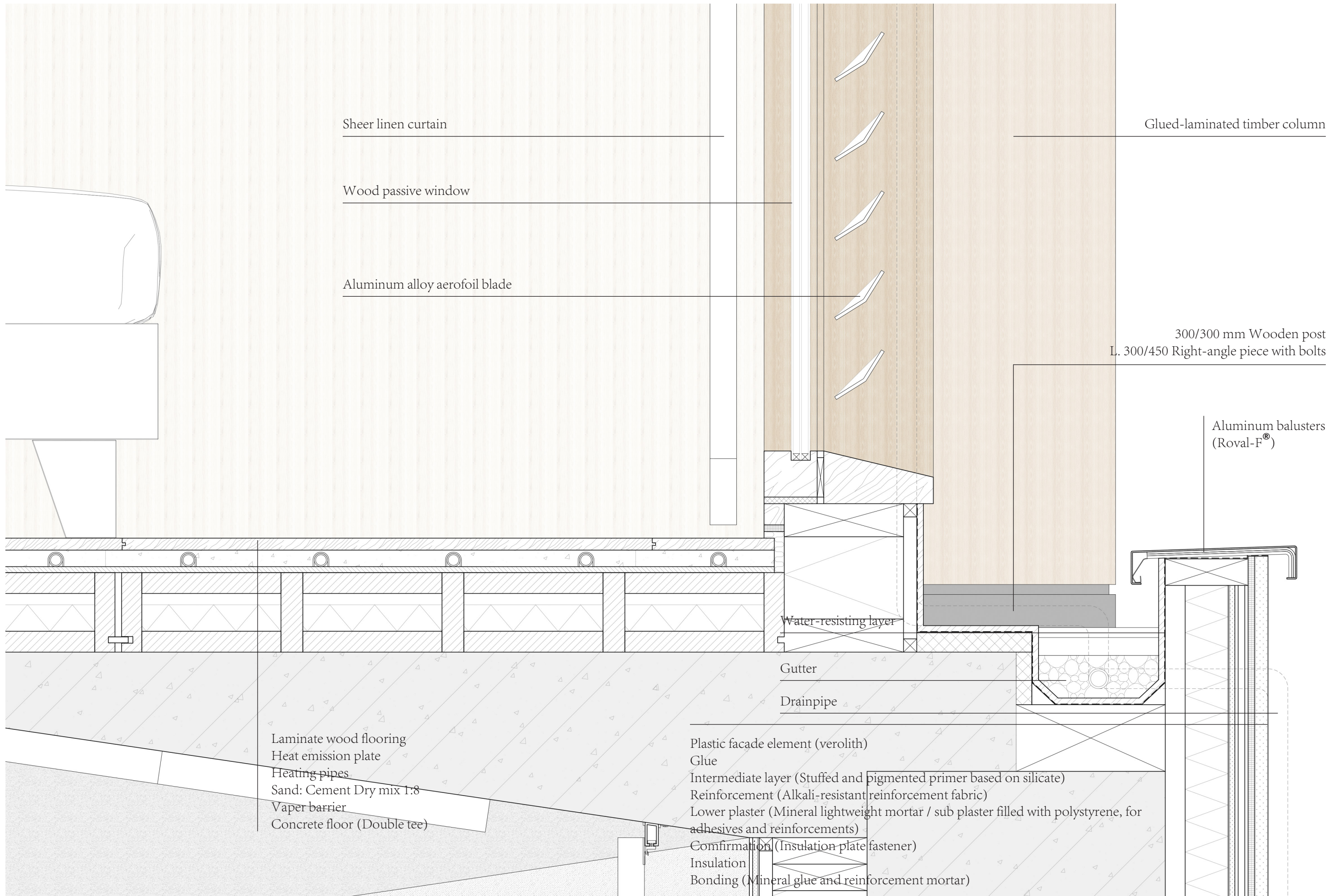
Detail 6 1:5
