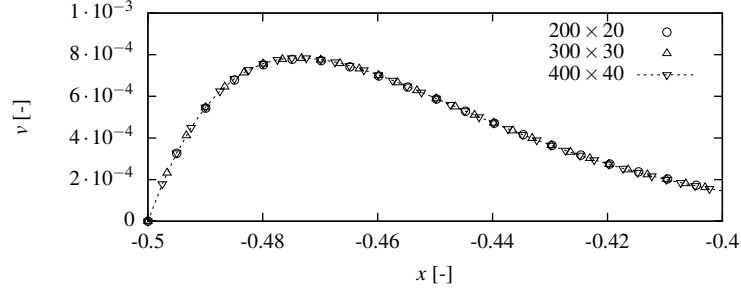
Figure 4: The vertical velocity component along the line y = 0.5 for A = 0.1 , Re = A , Ha^2 = 1 , Bo = A^2 , Ca = A^4 for mesh resolutions of 200 \times 20 , 300 \times 30 and 400 \times 40 .
