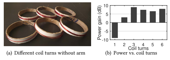
Figure 14: Power vs. turns of bracelet without any body part: (a) Coils with turns from one to six; (b) Harvested average power from coils with different turns.
