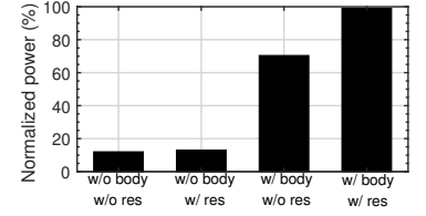
Figure 18: Normalized harvested power with four different harvesting setups.
