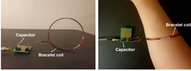
(a) Implemented energy harvesting antenna of Bracelet+
