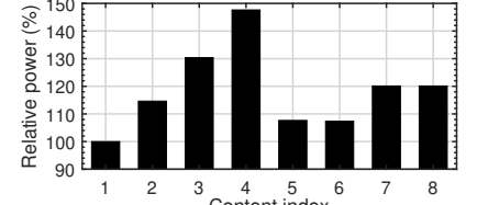
(b) Harvested power vs. Tx data
