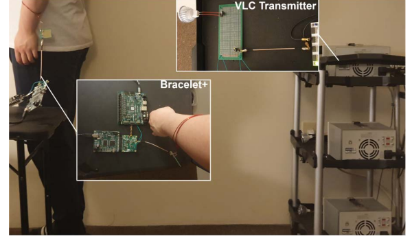
Figure 16: Experiment setup, including the energy harvesting system (bracelet+ front-end and energy measuring ADC circuit) and the VLC transmitters.
