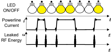
Figure 2: Illustration of the leaked RF energy caused by the power-line current change in VLC. Here we use OOK modulation as the example.
