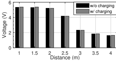
Figure 20: Measured VLC signals' maximum voltages with/without Bracelet+ harvesting energy.
