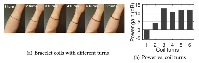
Figure 12: Power vs. turns of bracelet: (a) Bracelet coils with turns from one to six at a step size of one; (b) Average power of the received leaked energy from bracelet coils with different turns.
