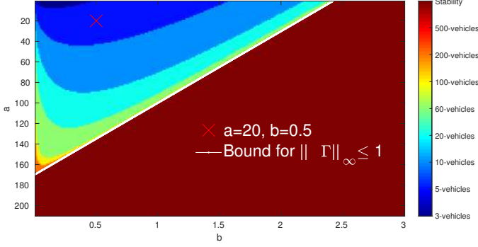
Fig. 5: Stability of (20)-(21) in the (a, b) -plane, when changing N (c.f. color bar on the right). The stability region decreases when increasing N . For N \rightarrow \infty the region tends to the sufficient condition (22), represented by a white line (the region above this line corresponds to \|\Gamma\|_\infty > 1 ).
