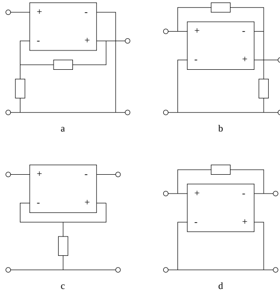
Figure 2: the possible amplifier configurations: (a) voltage amplifier, (b) current amplifier, (c) voltage-to-current amplifier, and (d) current-to-voltage amplifier.
