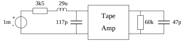
Figure 6: the environment of the tape amplifier.
