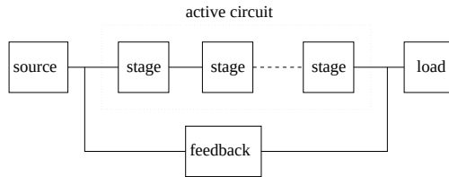
Figure 1: the general amplifier configuration used by Ampdes.
