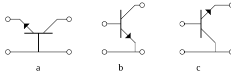
Figure 3: the possible stage configurations: (a) CB stage, (b) CE stage, (c) CC stage.
