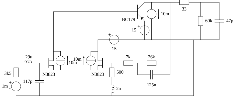
Figure 7: the tape amplifier designed by Ampdes.
