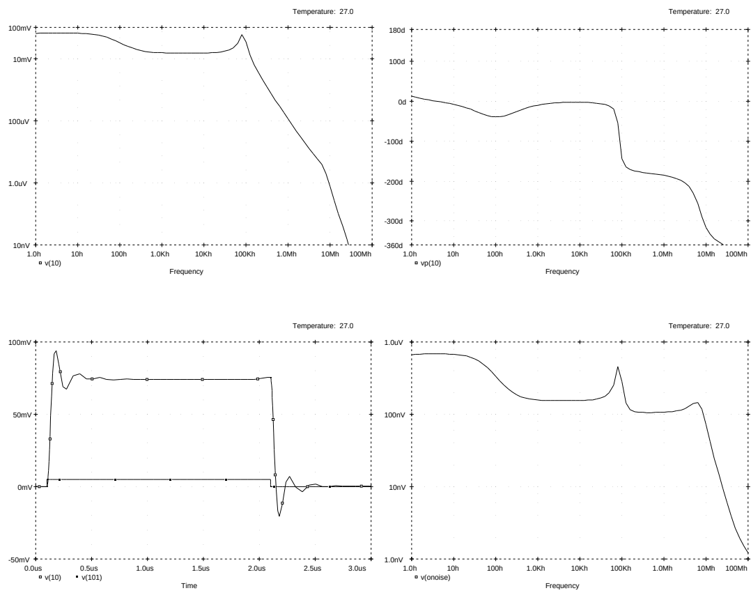
Figure 8: Some simulation results for the amplifier designed by Ampdes: the magnitude and phase plot of the transfer function of the amplifier, the transient response and the noise spectrum at the output.
