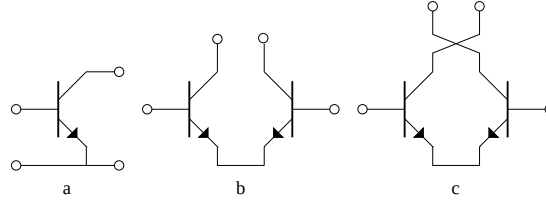
Figure 4: the possible variations on the stage configuration (shown for a CE stage): (a) single, (b) balanced, (c) non-inverting balanced.
