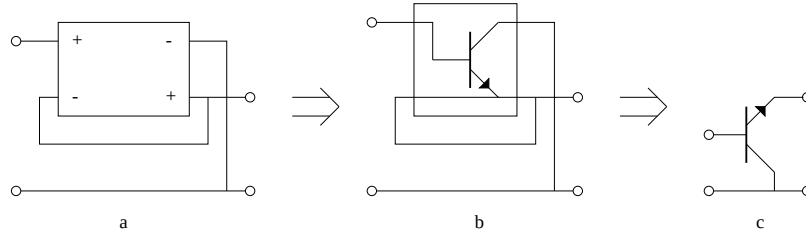
Figure 5: derivation of a CC stage from a CE stage (shown for an NPN transistor): (a) unity gain voltage amplifier (voltage follower), (b) unity gain amplifier with single CE stage (c) rearranged version of (b): a CC stage.
