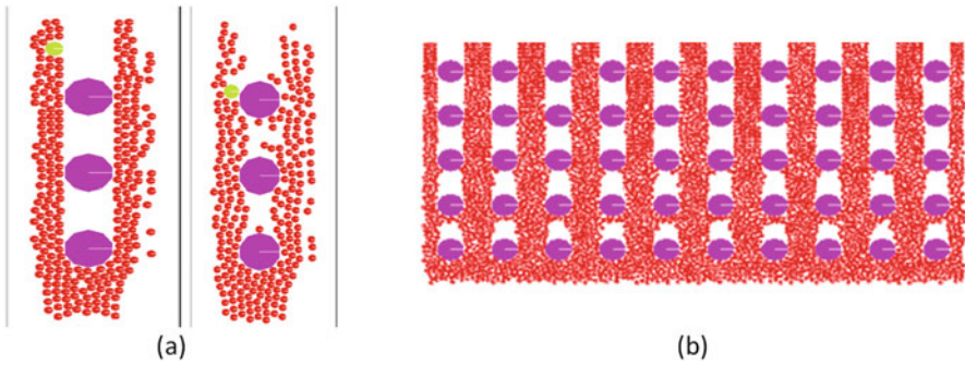
Fig. 4.29 DEM flow around bumps showing the impact of adhesive forces, flow direction is bottom to top; (a) left, no adhesive forces used; (a) right, moderate adhesion added; (b) no adhesive forces used in a full bump array. The solder bumps are represented by the large circles, and the filler particles are represented by the small circles
