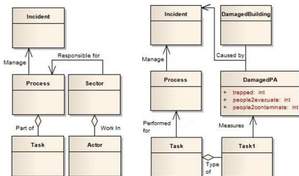
Figure 3. Conceptual diagram of top-level classes involved in DR in the Netherlands. Adopted from (Xu et al., 2008).
