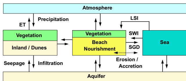
Figure 14. Hydrological, morphological, and ecological processes (arrows) that affect the growth of fresh groundwater resources in a (large) beach nourishment (LSI = land-surface inundations, ET = evapotranspiration, SGD = submarine groundwater discharge, and SWI = seawater intrusion).
