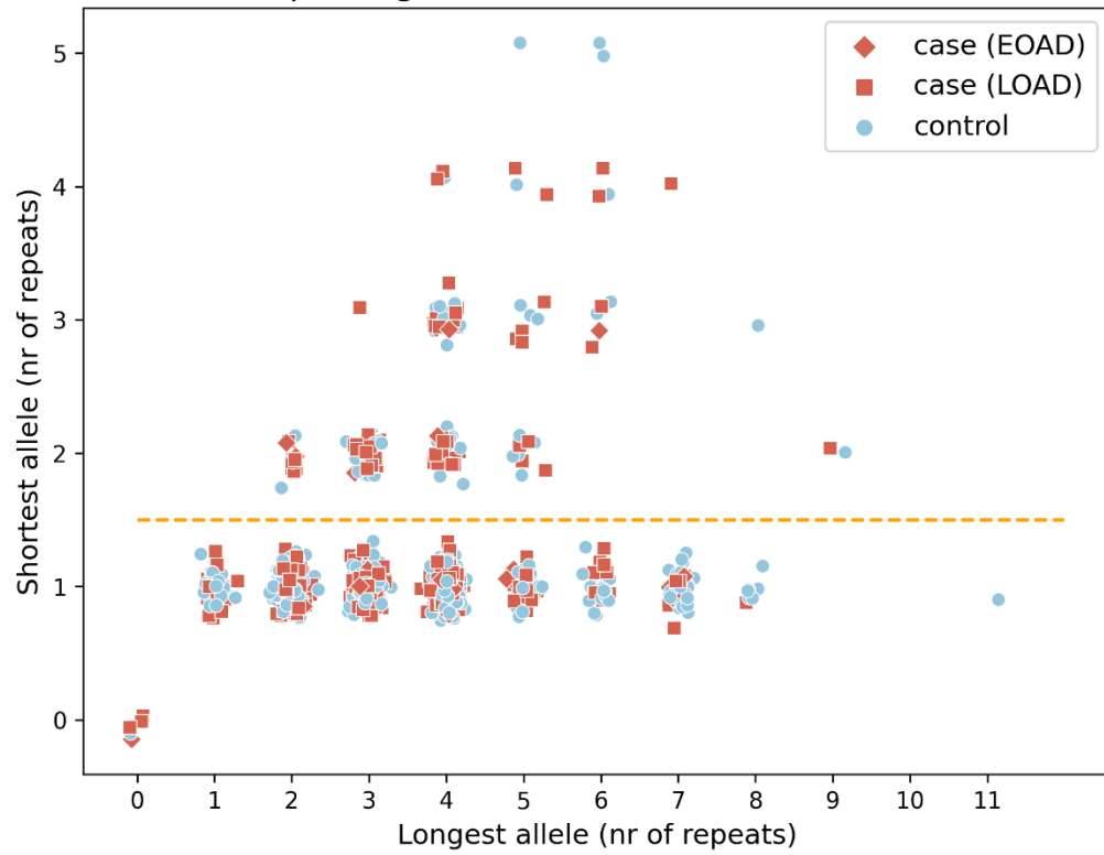
Supplementary Figure 2b: The excluded VNTR in the GALNT17 gene due to insufficient separation between cases and controls.
