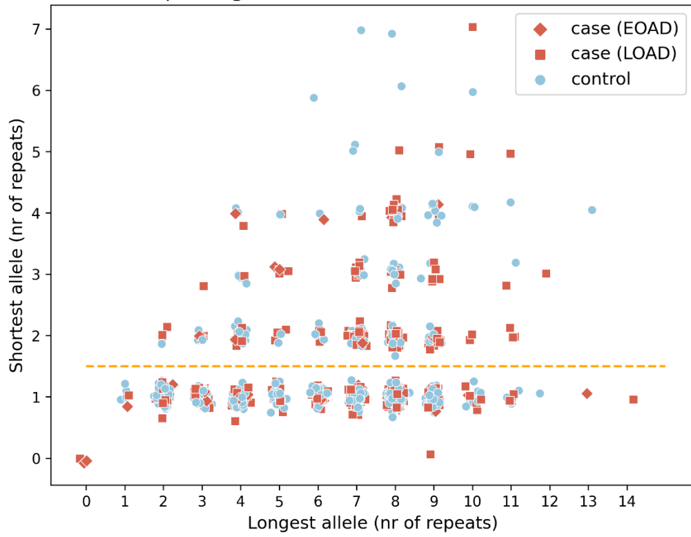
Supplementary Figure 2a: The excluded VNTR in the DLGAP2 gene due to insufficient separation between cases and controls.
