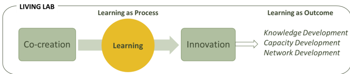
Figure 3. Co-creation- innovation-learning model for living labs
