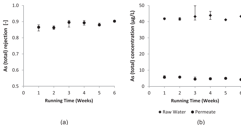
Fig. 4. (a) As rejection and (b) As concentration in feed water and permeate for the evaluated period.
