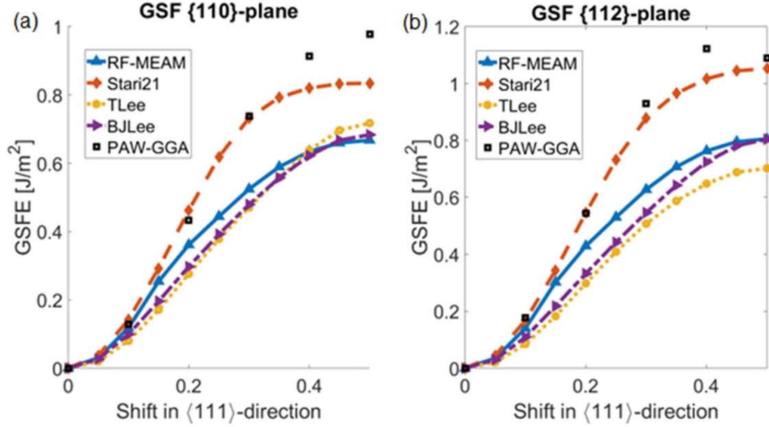
Figure 3. GSFE for the {110} and {112}-planes. A shift is introduced in the \langle 111 \rangle -direction. The solid lines belong to the RF-MEAM potential, the dashed lines to Stari21 , the dotted lines to TLee , and the dash-dotted lines to BJLee . The black squares are DFT results using PAW-GGA taken from [69]. The outlier here is Stari21 which produces a consistently high surface and USF energy too.
