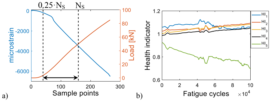
Fig. 5. a) Indicative samples of FBG strain readings and test machine's compressive load, b) evolution of HIs for L1_23.
